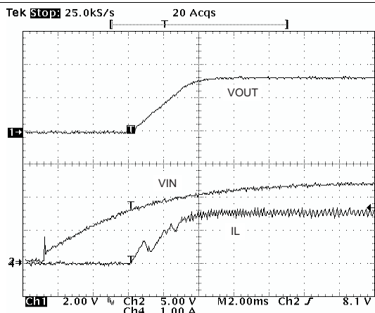
Figure 42. VIN Power Up
