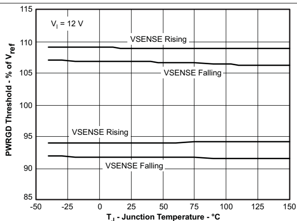
Figure 20. PWRGD Threshold vs Junction Temperature
