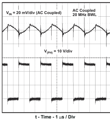
图 7-6. Output Voltage Ripple and PH Node, I_O = 1\text{ A}
