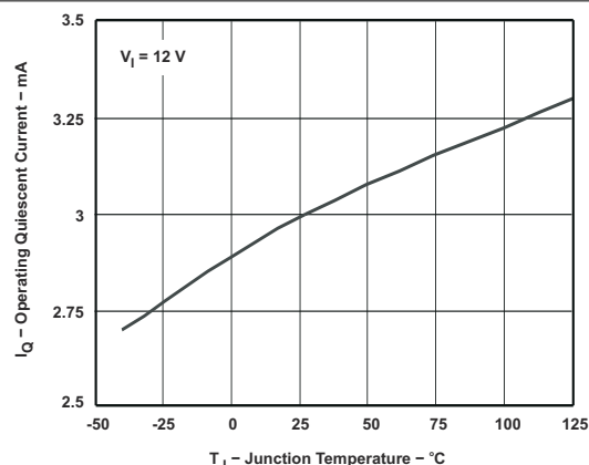
图 5-2. Operating Quiescent Current vs Junction Temperature
