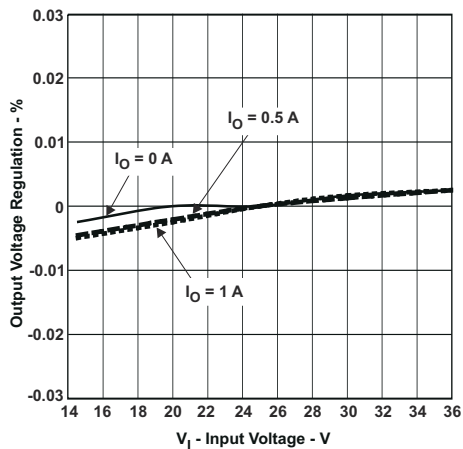
图 7-4. Output Voltage Regulation % vs Input Voltage
