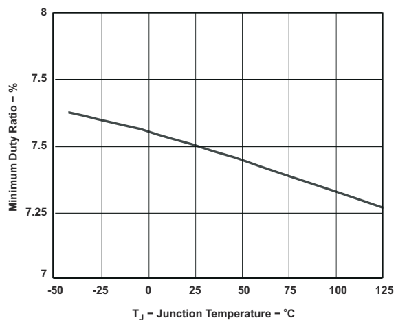
图 5-8. Minimum Controllable Duty Ratio vs Junction Temperature
