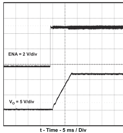
图 7-9. Start-up Waveform, ENA and V_O
