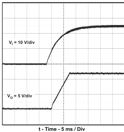
图 7-8. Start-up Waveform, V_I and V_O
