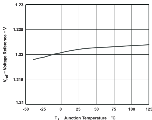
图 5-4. Voltage Reference vs Junction Temperature
