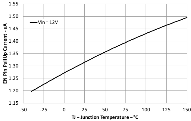
图 7-7. EN Pin Pullup Current vs Junction Temperature, V_{\text{EN}} = 1.1\text{ V}
