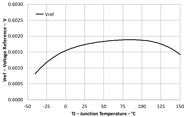
图 7-3. Voltage Reference vs Junction Temperature
