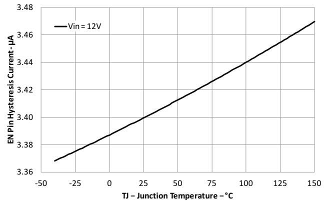
图 7-6. EN Pin Hysteresis Current vs Junction Temperature, V_{EN} = 1.3\text{ V}
