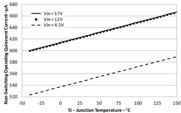
图 7-9. Nonswitching Operating Current vs Junction Temperature
