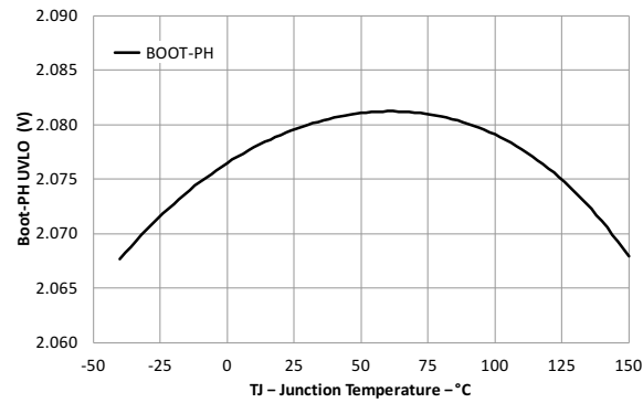
图 7-15. BOOT-PH UVLO vs Junction Temperature
