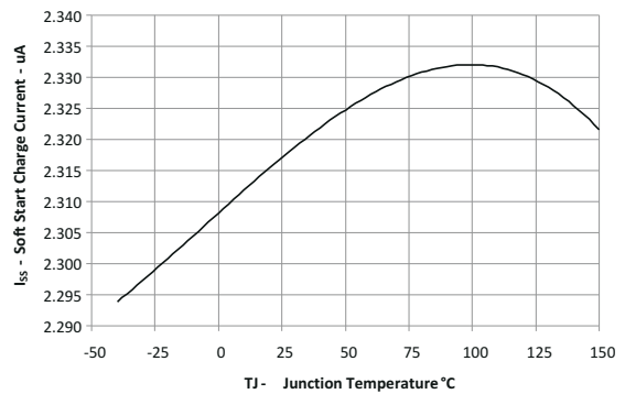
图 7-10. Soft-Start Charge Current vs Junction Temperature
