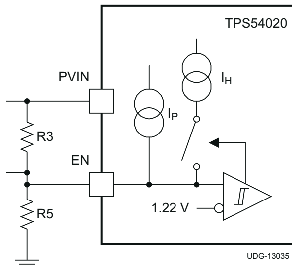
图 8-2. Adjustable PVIN Undervoltage Lockout, PVIN \geq 4.5 \text{ V}
