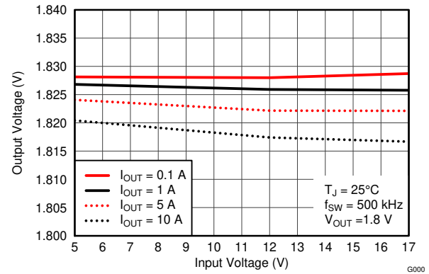
图 9-13. Line Regulation
