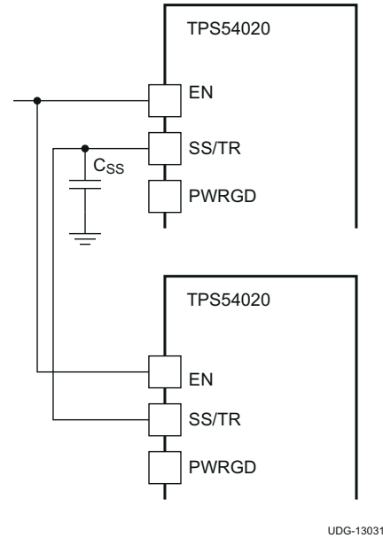
图 8-5. Ratiometric Start-up Sequence
