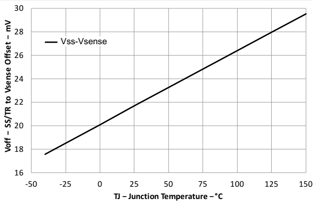
图 7-11. (V_{\text{SS}} - V_{\text{VSENSE}}) Offset vs Junction Temperature
