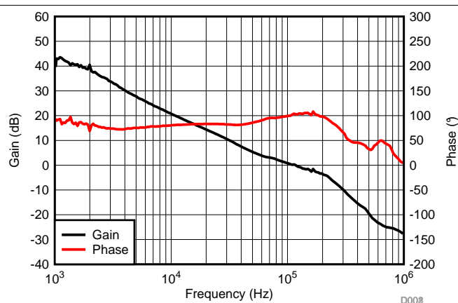
Figure 95. Bode Plot
