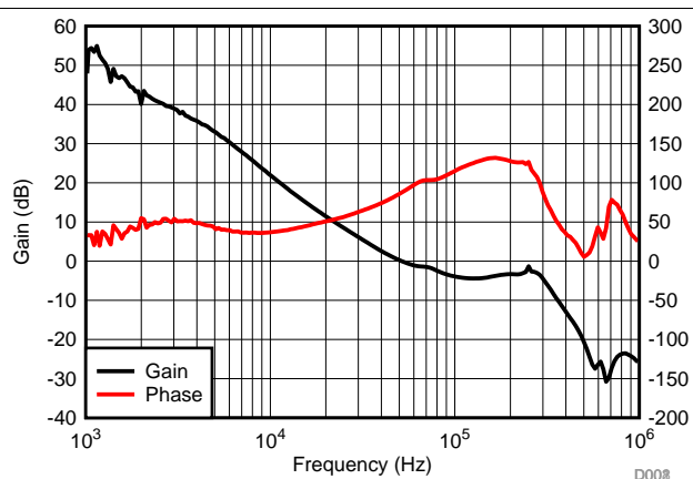
Figure 94. Bode Plot
