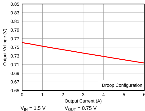
图 27. Load Regulation (Droop Configuration)
