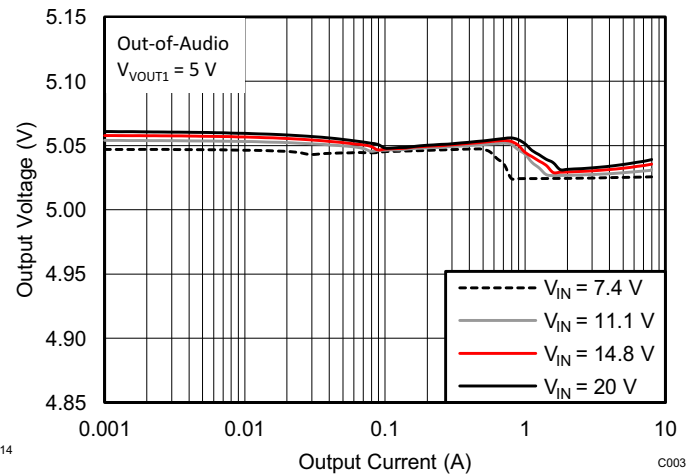
Figure 14. Load Regulation
