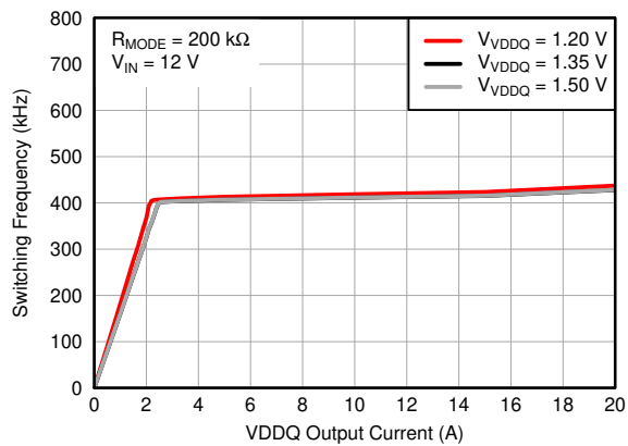
图 7-12. Switching Frequency vs Load Current
