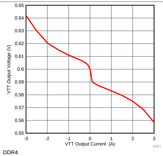
Figure 16. VTTREF Output Voltage vs Output Current
