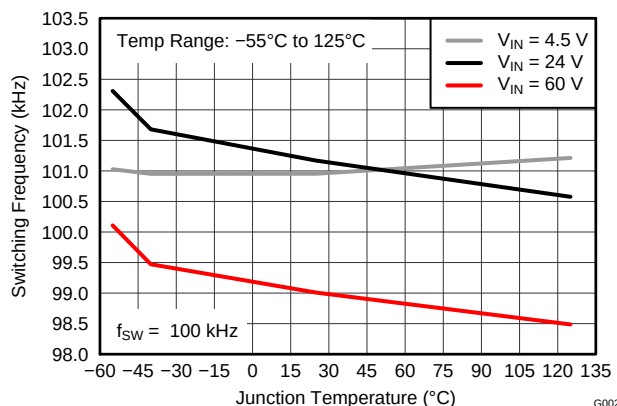
Figure 3. Switching Frequency vs Junction Temperature (f sw = 100 kHz)
