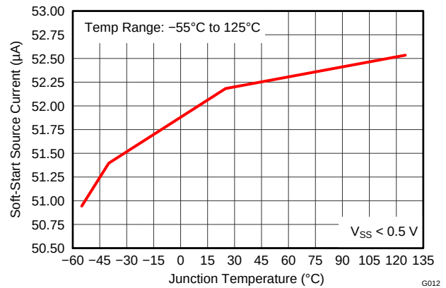
Figure 13. Soft-Start Source Current vs Junction Temperature ( V_{SS} < 0.5 \text{ V} )
