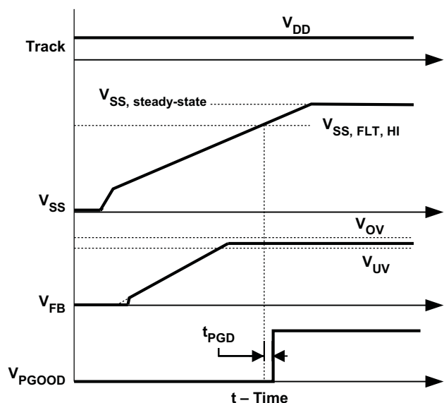
Figure 35. PGOOD Signal
