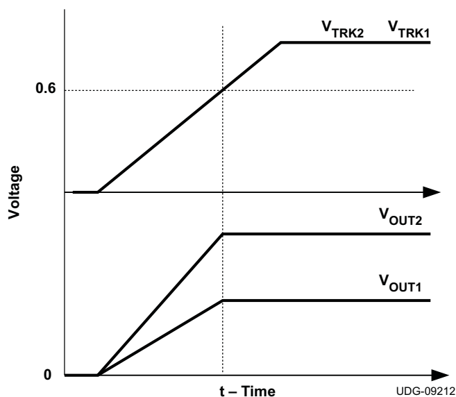
Figure 30. Ratiometric Voltage-Tracking Schematic Figure 31. Ratiometric Voltage-Tracking Waveform
