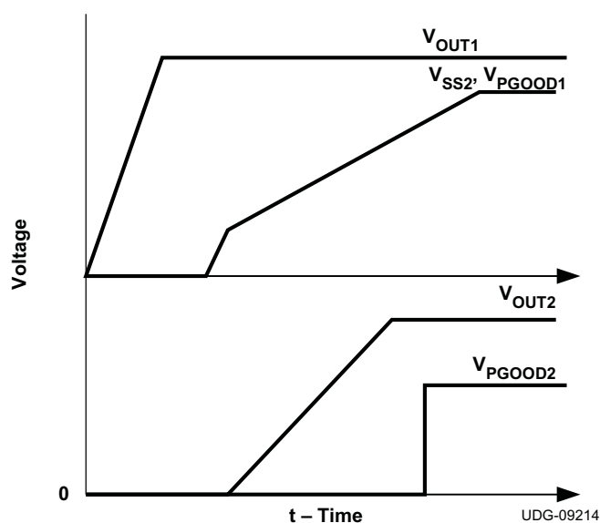
Figure 33. Sequential Start-Up Waveform
