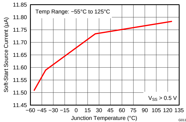
Figure 12. Soft-Start Source Current vs Junction Temperature ( V_{SS} > 0.5 \text{ V} )
