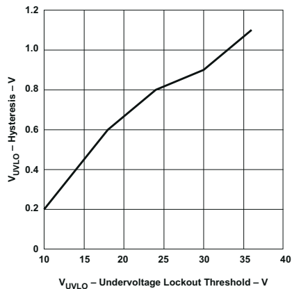
图 6-3. Undervoltage Lockout Threshold vs Hysteresis
