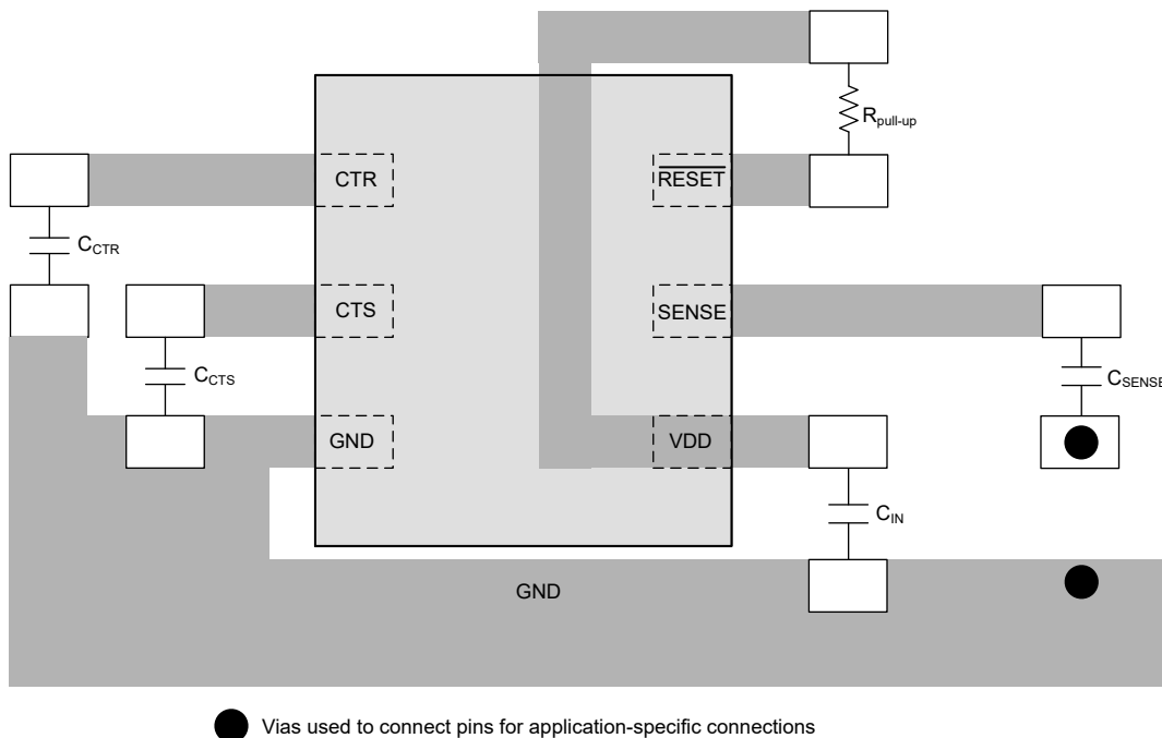
图 7-5. Recommended Layout
