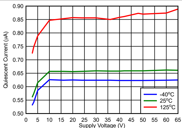
RESET = Low, V_{IT} = 2.7\text{ V} 图 7-5. V_{DD} vs I_{DD} (RESET = Low, V_{IT} = 2.7\text{ V} )
