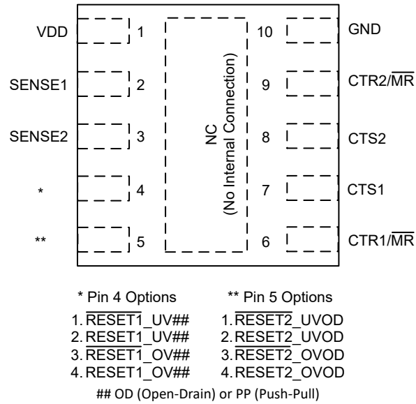
图 6-1. DSK Package, 10-Pin WSON, TPS38 (Top View)
