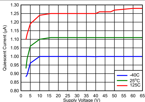
RESET = High, V_{IT} = 0.8\text{ V} 图 7-6. V_{DD} vs I_{DD} (RESET = High, V_{IT} = 0.8\text{ V} )
