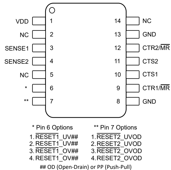
图 6-2. DYY Package, 14-Pin SOT-23, TPS38 (Top View)
