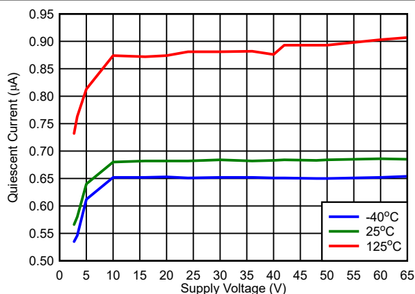
RESET = High, V_{IT} = 2.7\text{ V} 图 7-4. V_{DD} vs I_{DD} (RESET = High, V_{IT} = 2.7\text{ V} )
