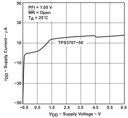
图 7-3. Supply Current vs Supply Voltage
