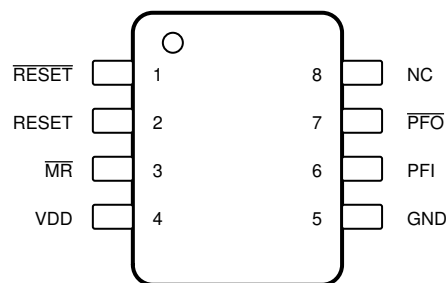
图 6-4. TPS3707-xx DGN Package 8-Pin MSOP-PowerPAD Top View
