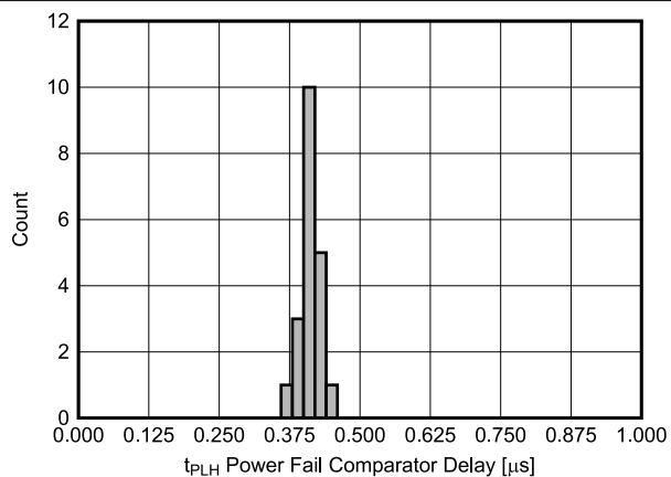
图 7-25. PFI to PFO (t PHL ) Delay Histogram for TPS3705-33 Devices at 25°C (Unit Count = 20)
