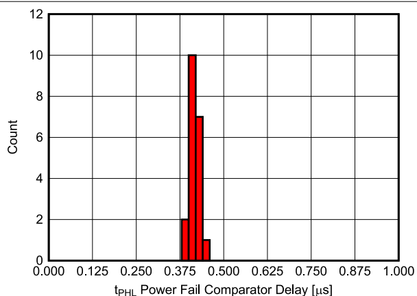
图 7-23. PFI to PFO (t PHL ) Delay Histogram for TPS3705-33 Devices at 125°C (Unit Count = 20)
