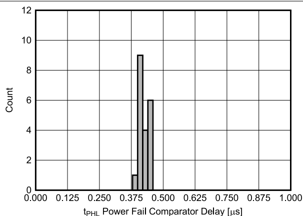
图 7-22. PFI to PFO (t PHL ) Delay Histogram for TPS3705-33 Devices at 25°C (Unit Count = 20)
