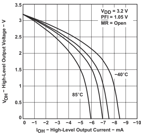
图 7-6. High-Level Output Voltage vs High-Level Output Current
