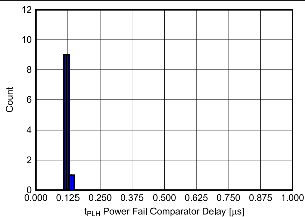
图 7-24. PFI to PFO (t PHL ) Delay Histogram for TPS3705-33 Devices at -40°C (Unit Count = 20)
