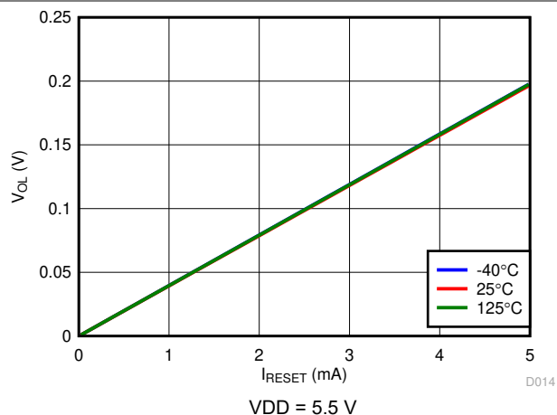
图 7-16. Low-Level Output Voltage vs RESET current
