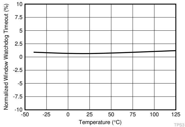
图 6-7. Normalized Watchdog Timeout ( t_{WD} ) Accuracy (SET1 = 1, CWD = 10\text{k}\Omega )
