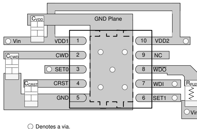
图 10-1. Typical Layout for the TPS3430
