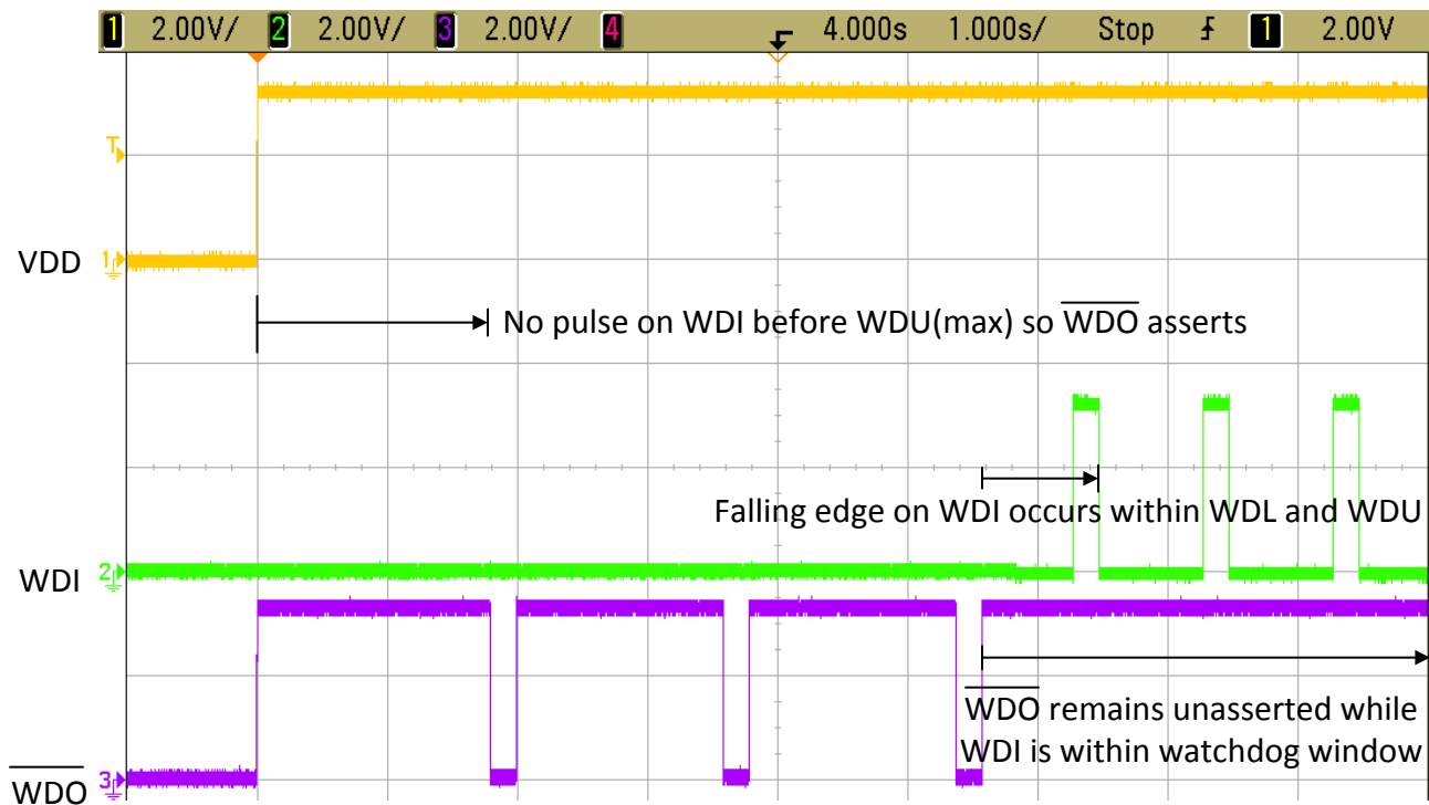
图 8-4. Watchdog Fault Caused by Missing WDI Pulse Until WDI pulses Arrive Within Watchdog Window to Deactivate \overline{WDO} Fault
