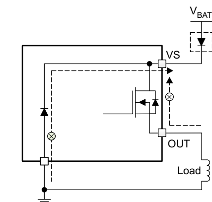
Figure 35. Reverse-Current External Protection, Method 1
