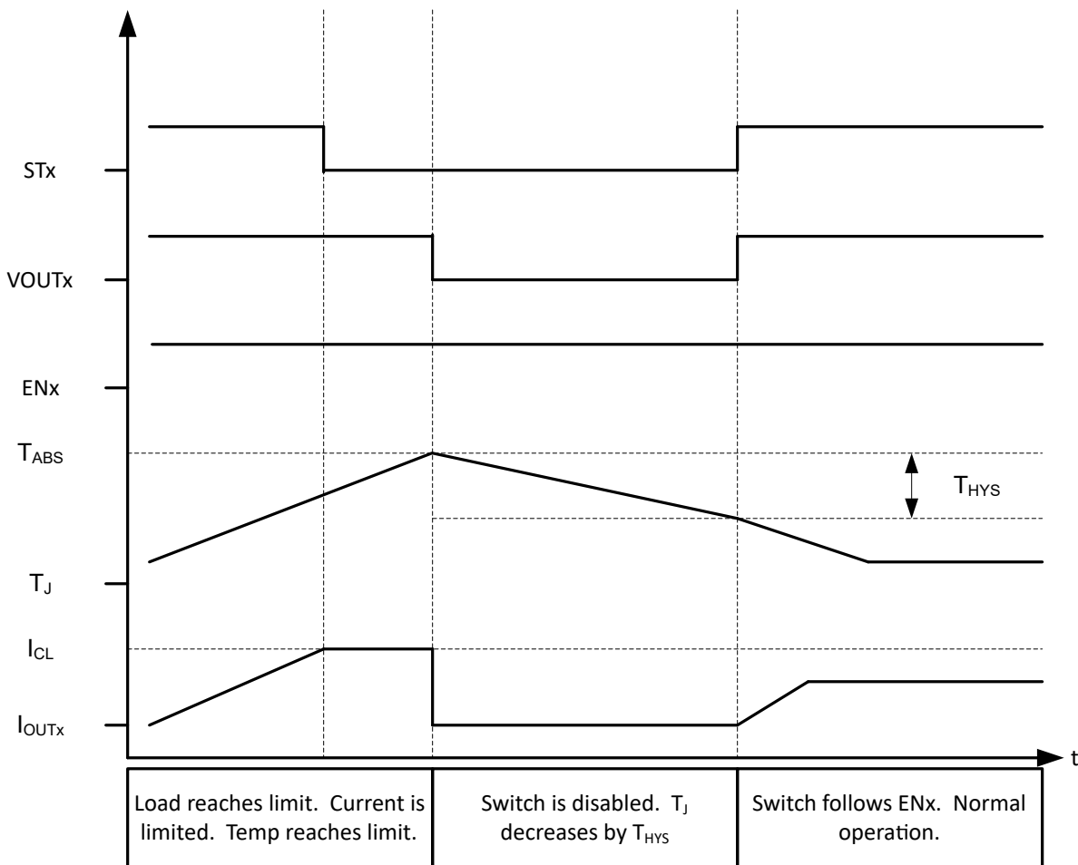
Figure 8-9. Thermal Shutdown - Auto-retry Behavior
