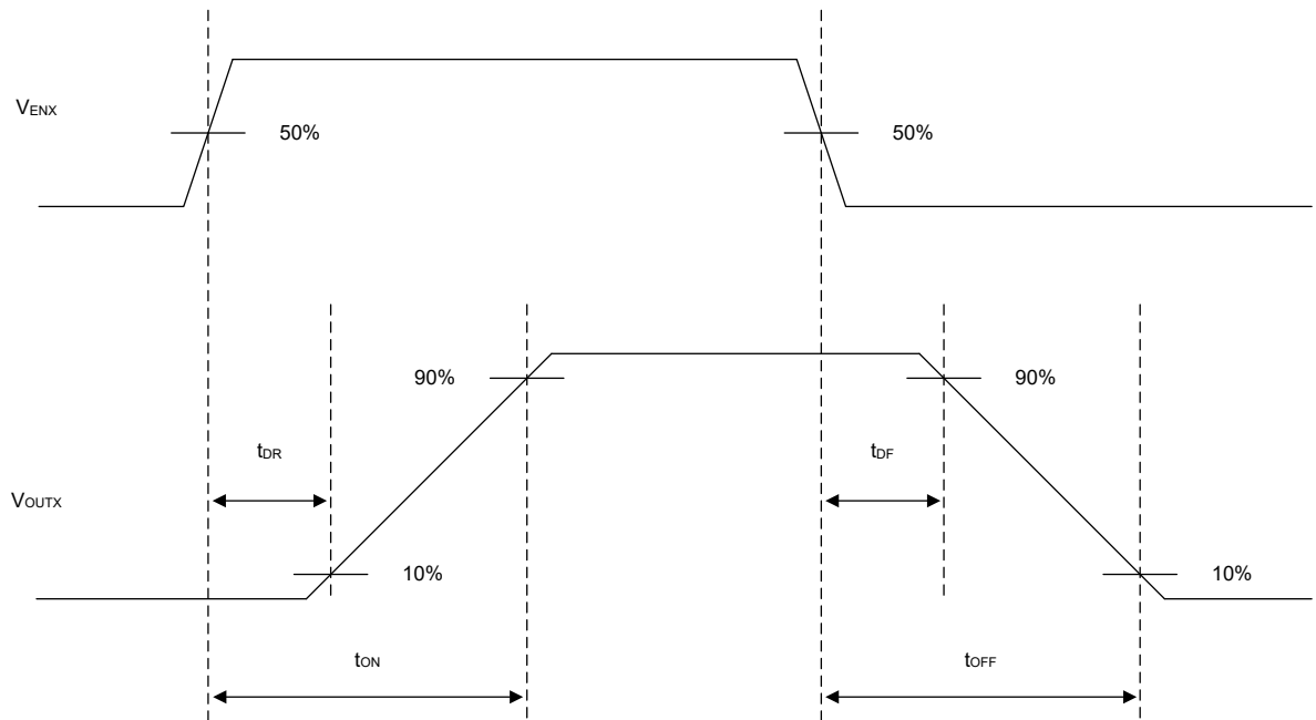
Figure 7-1. Switching Characteristics Definitions
