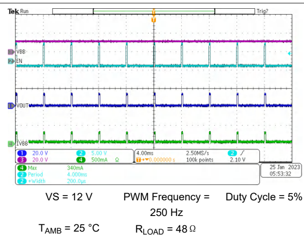
图 6-4. Switching the Part With 250-Hz PWM Signal
