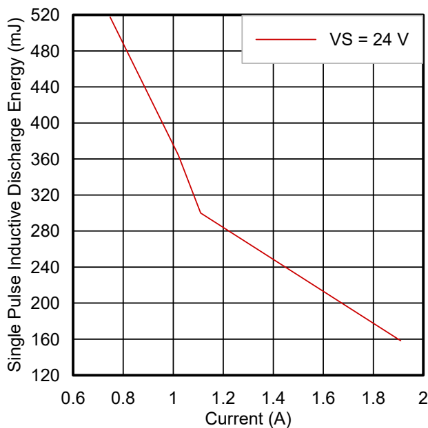
图 8-27. Maximum Energy Dissipation ( E_{AS} ) Allowed T_{J, START} = 125^{\circ}\text{C} – Single Pulse, One Channel
