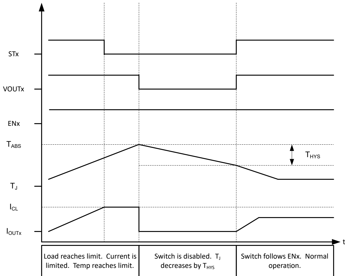
图 8-33. Current Limit - \text{AUTO\_RETRY\_DIS} = 0
