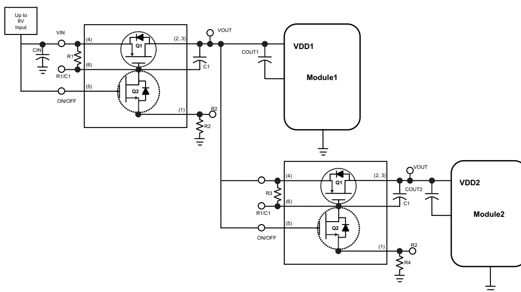
Figure 9. Power Sequencing using TPS27081A, Example 3
