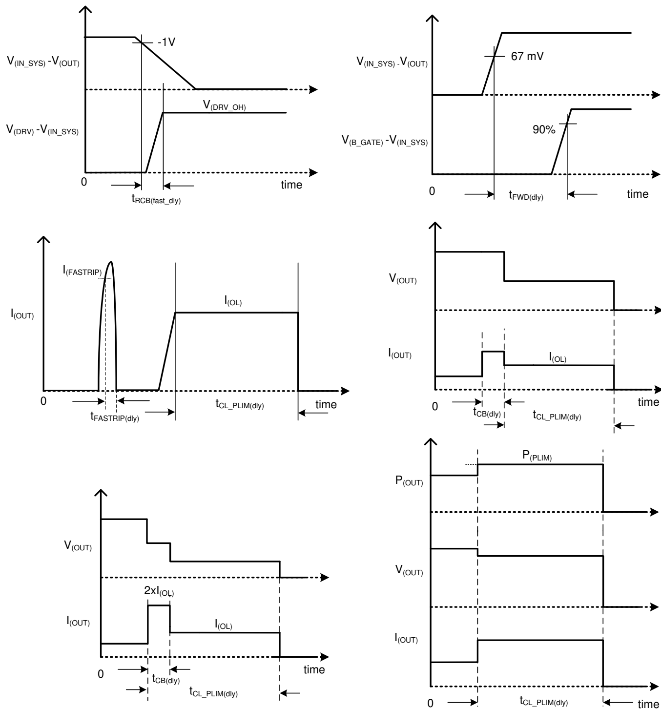
图 7-2. Timing Waveforms
