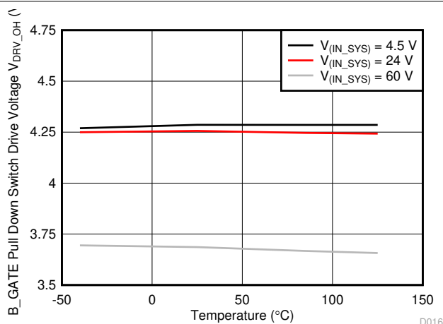
图 6-5. B_GATE Pulldown Drive Voltage vs Temperature
