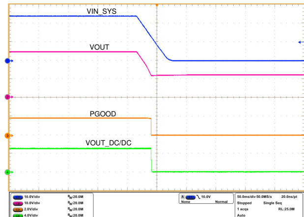
图 9-8. Power-Down Response
