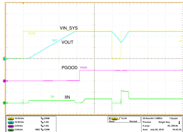
图 9-6. Power Up Followed with Voltage Interruption with TPS26630
