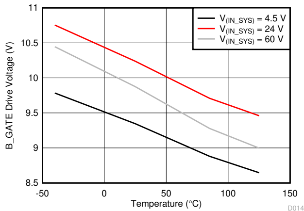
图 6-3. B_GATE Drive Voltage vs Temperature
