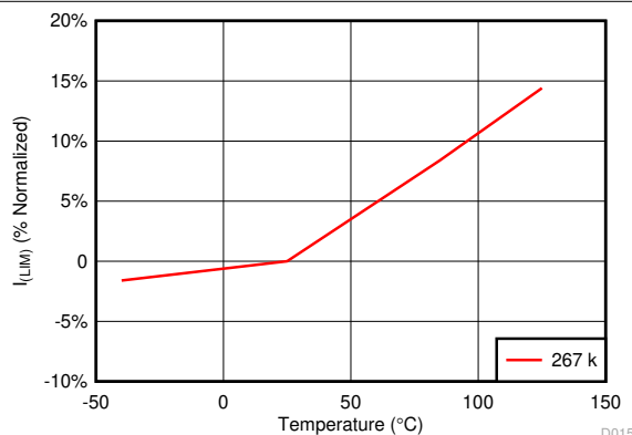
图 7-16. Current Limit (% Normalized) vs Temperature
