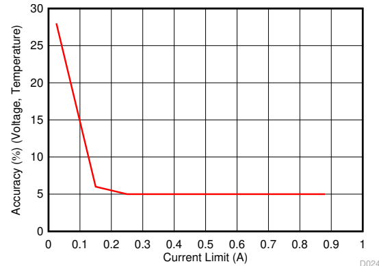
图 7-20. Current Limit Accuracy vs Current Limit, I_{\text{OL}}
