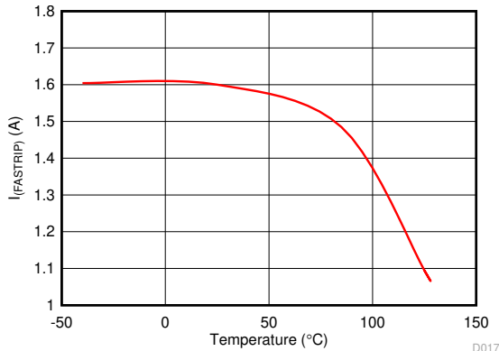
图 7-19. Fast-Trip Comparator Threshold I_{\text{FAST-TRIP}} vs Temperature Threshold
