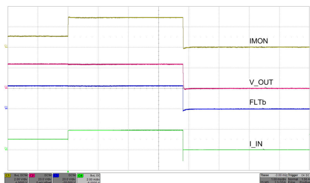
Load Transition from 22 Ω to 12 Ω , R_{ILIM} = 8 \text{ k}\Omega
