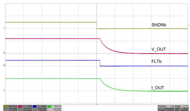
图 7-30. Turnoff Control With \overline{SHDN}
