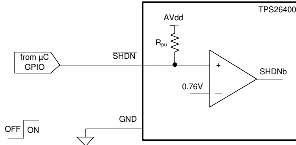
图 9-17. Shutdown Control
