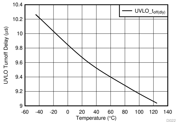
图 7-24. UVLO Turnoff Delay vs Temperature
