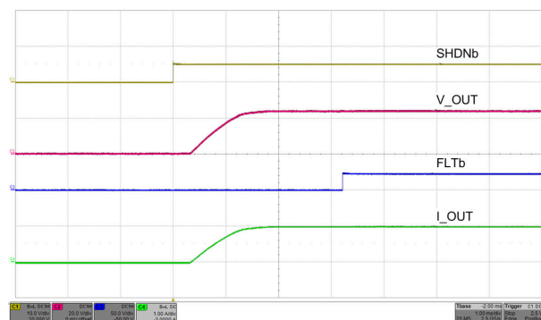
图 7-29. Turnon Control With \overline{SHDN}
