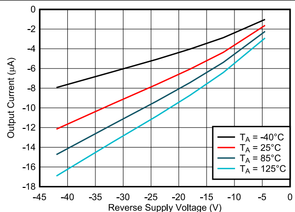
图 7-12. Output Current vs Reverse Supply Voltage, -V_{(\text{IN})}
