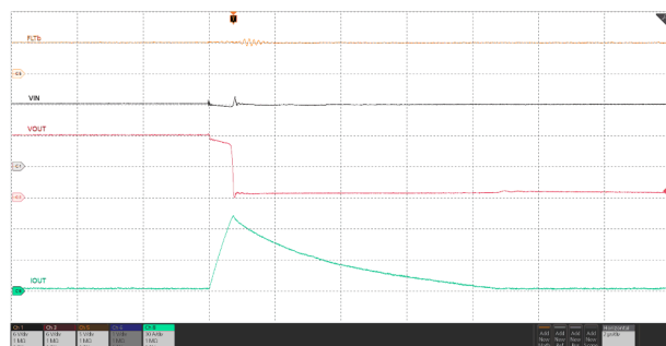
图 6-43. Circuit-Breaker Response TPS25974x
