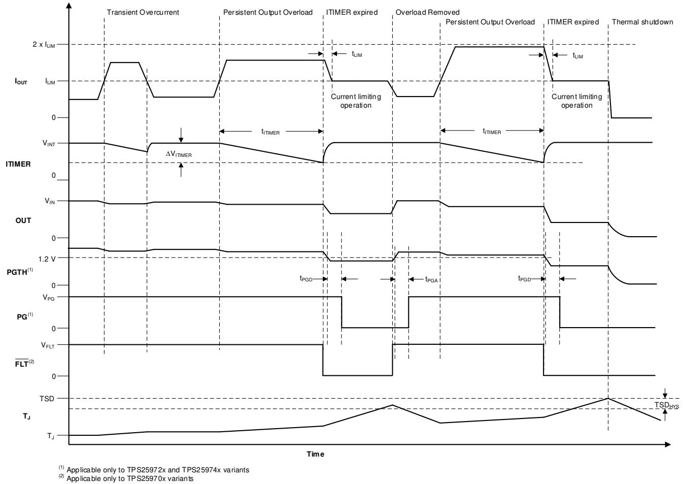
图 7-10. TPS25970x and TPS25972x Active Current Limit Response
