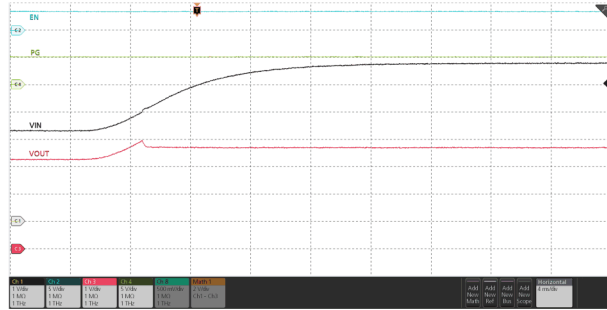
ROVSEL = GND, C_{OUT} = 220 \mu F , I_{OUT} = 200 mA , V_{IN} ramped up from 3.3 V to 5.8 V
