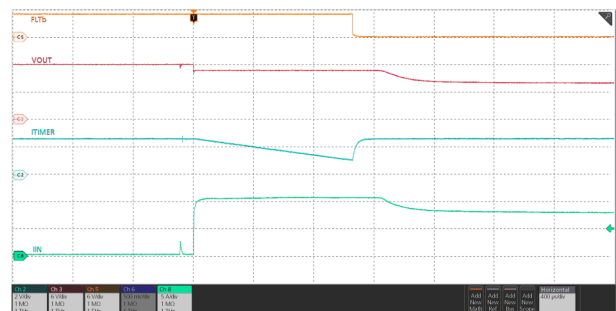
V_{IN} = 12 V , C_{TIMER} = 1.3 nF , C_{OUT} = 220 \mu F , R_{ILM} = 715 \Omega , I_{OUT} stepped from 0 A \rightarrow 11 A
