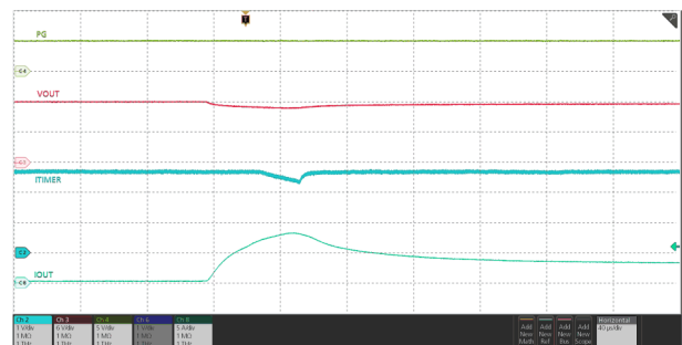
V_{IN} = 12 V , C_{TIMER} = 120 pF , C_{OUT} = 470 \mu F , R_{ILM} = 715 \Omega , I_{OUT} ramped from 0 A \rightarrow 8 A \rightarrow 4 A within 100 \mu s
