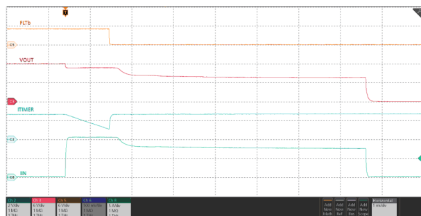
V_{IN} = 12 V , C_{TIMER} = 1.3 nF , C_{OUT} = 220 \mu F , R_{ILM} = 715 \Omega , I_{OUT} stepped from 0 A \rightarrow 11 A
