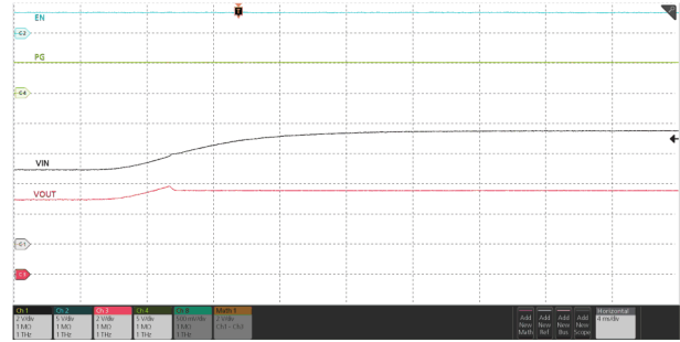
ROVSEL = Open, C_{OUT} = 220 \mu F , I_{OUT} = 200 mA , V_{IN} ramped up from 5 V to 7.5 V
