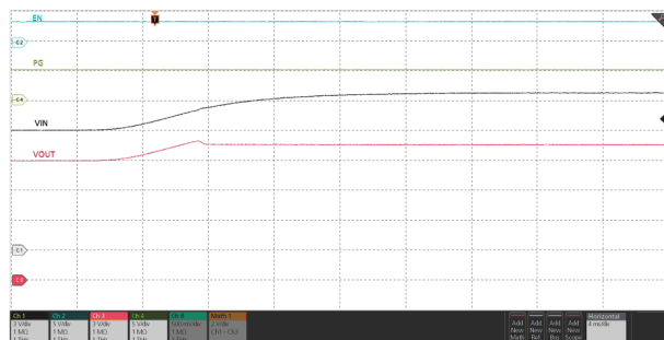
ROVSEL = 390 k \Omega , C_{OUT} = 220 \mu F , I_{OUT} = 200 mA , V_{IN} ramped up from 12 V to 16.5 V
