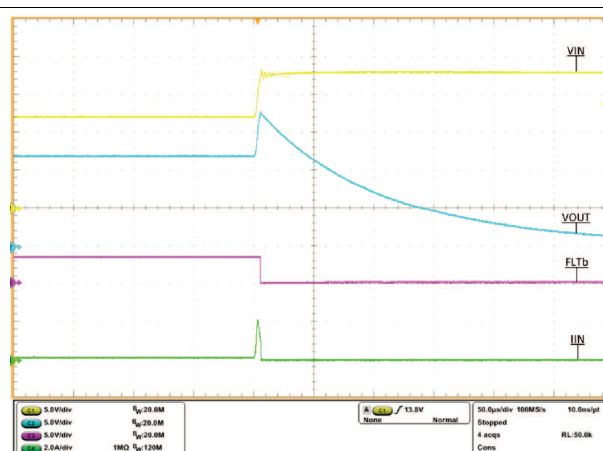
图 39. Hot Plug Response
