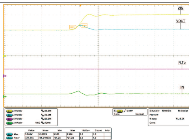
图 41. TPS259573 Overvoltage Lockout \overline{\text{FLT}} Response
