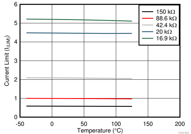
图 7-18. Current Limit vs Temperature Across R_{(\text{ILIM})}
