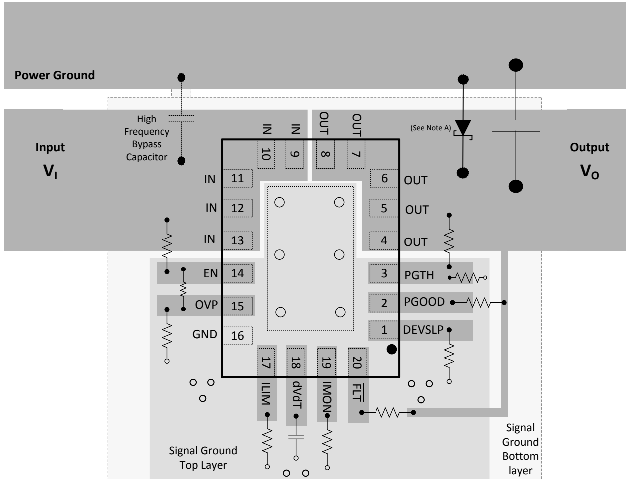
图 12-1. Board Layout
