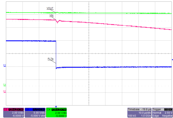
图 10-25. Hot-Plug Out Condition: FLT Delay
