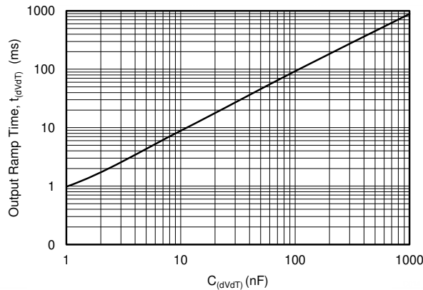
图 7-15. Output Ramp Time vs C_{(\text{dvdT})}
