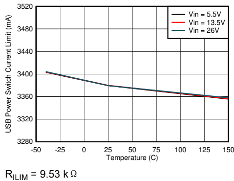
图 8-13. USB Power Switch Current Limit vs Junction Temperature
