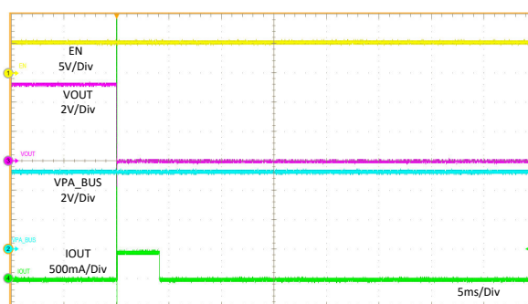
图 11-28. PA_CC2 Hot Short to GND
