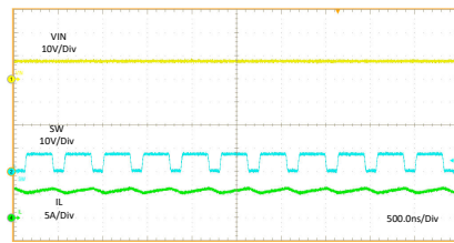
图 10-5. Switching Frequency When R_{FREQ} = 8.45 \text{ k}\Omega
