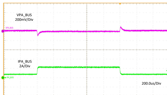
图 11-10. Load Transient Without Cable Compensation
