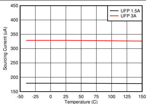
图 8-23. CC Sourcing Current vs Junction Temperature
