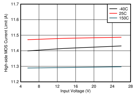
图 8-8. High-side Current Limit vs Input Voltage
