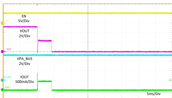
图 11-29. OUT Short to 5.1- \Omega Load
