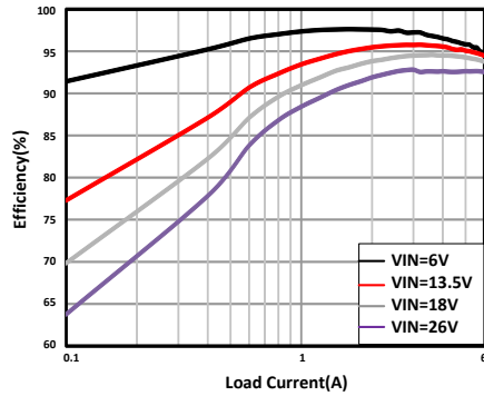
图 11-3. Buck Only Efficiency
