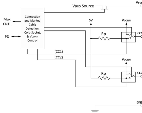
图 10-21. Source Functional Model for CC1 and CC2 (From Type-C Specification)
