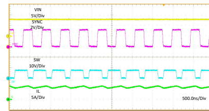
图 10-6. Switching Frequency When R_{FREQ} = 8.45 \text{ k}\Omega
