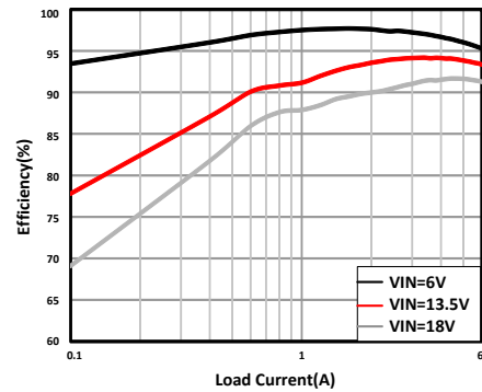
图 11-4. Buck Only Efficiency
