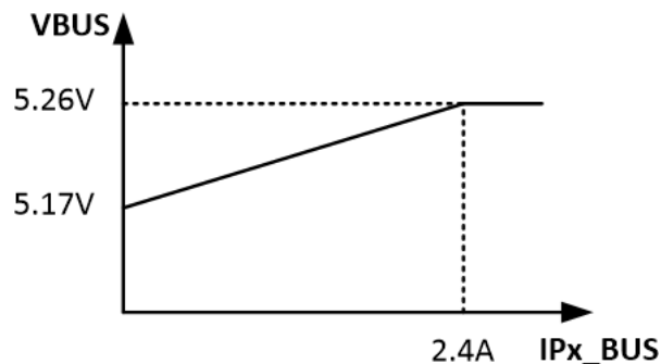
图 10-15. Dual Ports Cable Compensation
