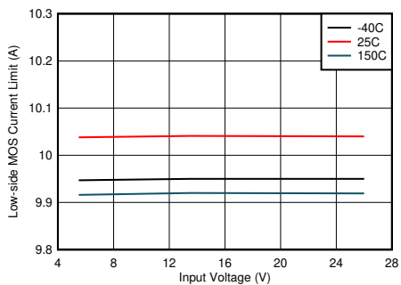
图 8-9. Low-side Current Limit vs Input Voltage
