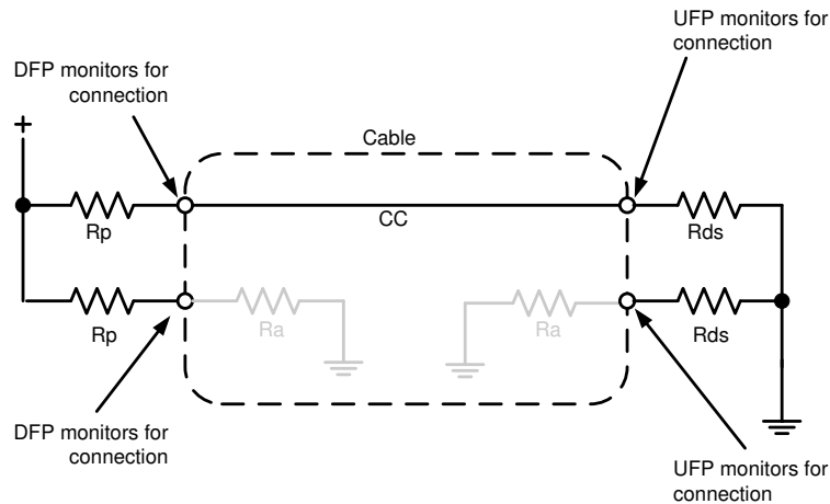
图 10-20. DFP-UFP Connection
