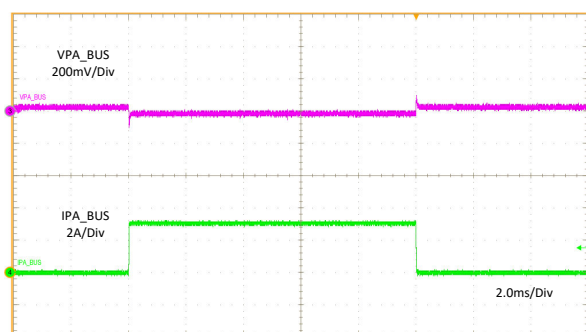
图 11-11. Load Transient With Cable Compensation
