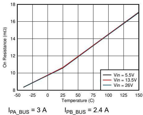
图 8-11. Low-side MOSFET on Resistance vs Junction Temperature
