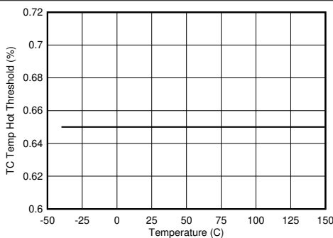
图 8-25. TS Temperature Hot Threshold vs Junction Temperature
