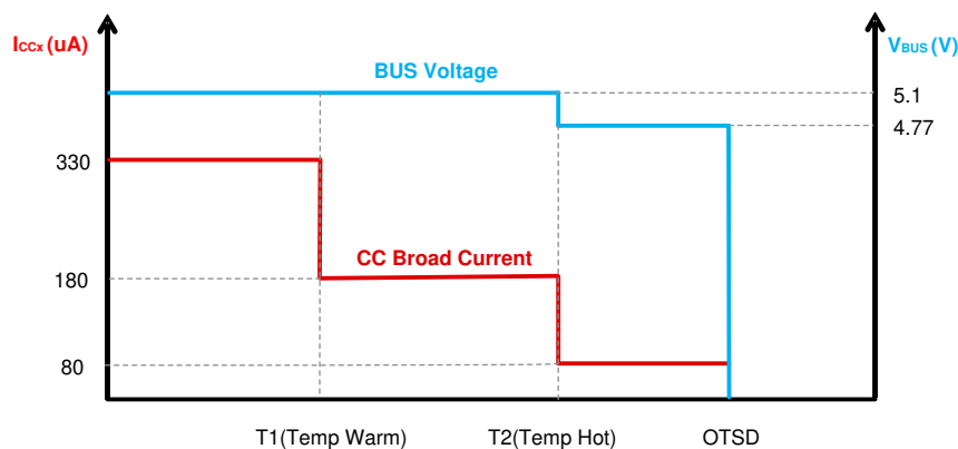
图 10-17. TPS2586x-Q1 Behavior When Trigger Temp Warm/Hot Threshold
