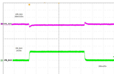
图 11-9. Load Transient Without Cable Compensation
