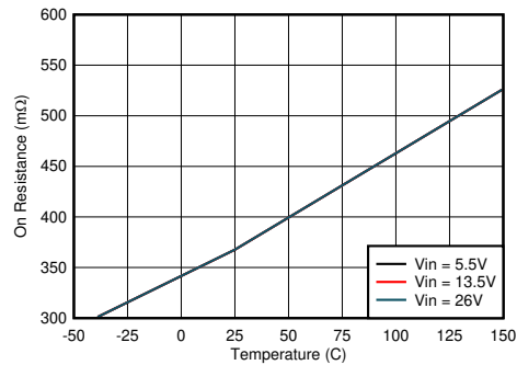
图 8-20. VCONN Power Switch On Resistance vs Junction Temperature
