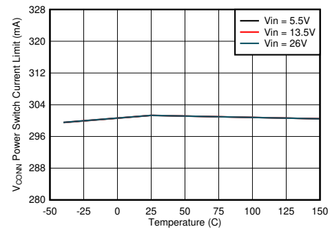
图 8-16. V_{CONN} Power Switch Current Limit vs Junction Temperature
