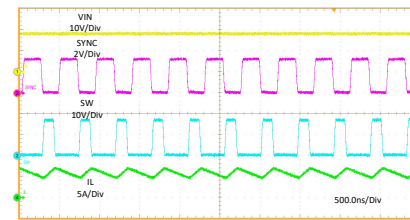
图 10-10. Synchronizing to External 2.2-MHz Clock
