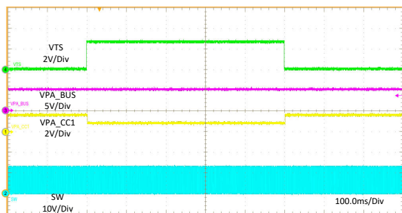
图 11-31. Thermal Sensing - NTC Temperature WARM Behavior
