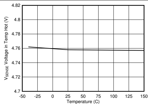
图 8-26. SENSE Voltage in Temperature Hot vs Junction Temperature
