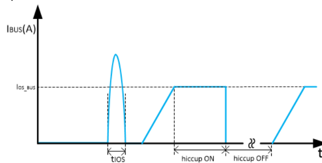
图 10-11. Response Time to BUS Short-Circuit
