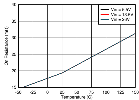
图 8-10. High-side MOSFET on Resistance vs Junction Temperature
