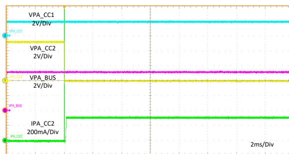
图 11-28. PA_CC2 Hot Short to GND
