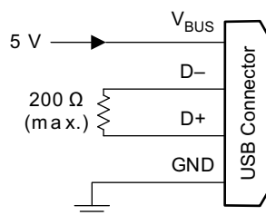
图 10-22. DCP Supporting BC1.2 and YD/T 1591-2009
