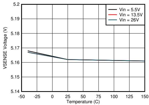
图 8-5. V_{SENSE} Voltage vs Junction Temperature
