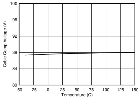
图 8-17. Cable Compensation Voltage vs Junction Temperature
