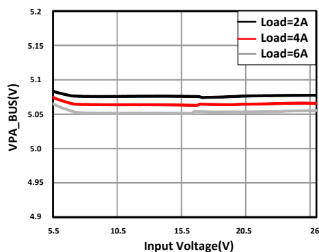
图 11-13. Dropout Characteristic
