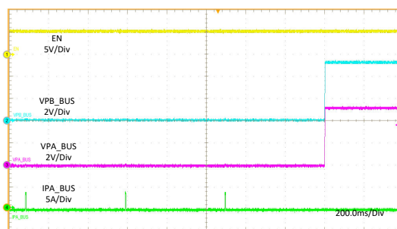
图 11-24. Short Circuit Recovery
