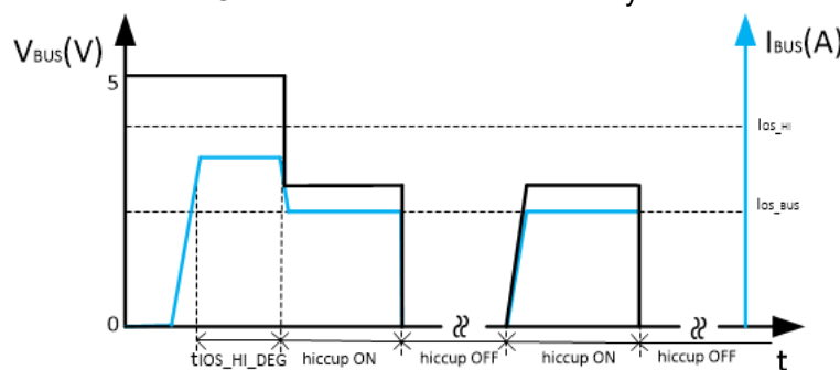
图 10-12. BUS Overcurrent Protection
