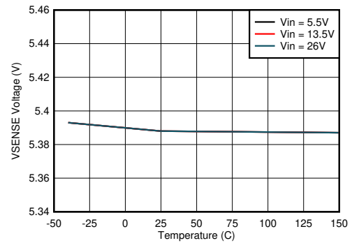
图 8-6. V_{SENSE} Voltage vs Junction Temperature
