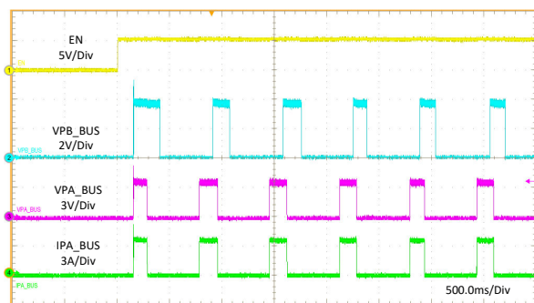
图 11-23. Enable Into Short
