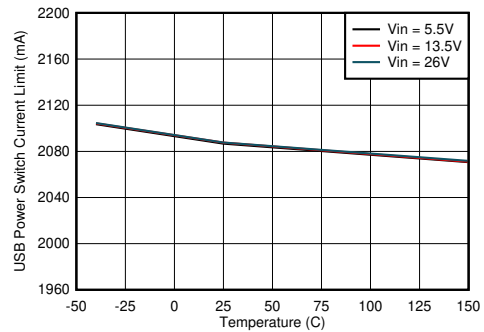
图 8-12. USB Power Switch Current Limit vs Junction Temperature
