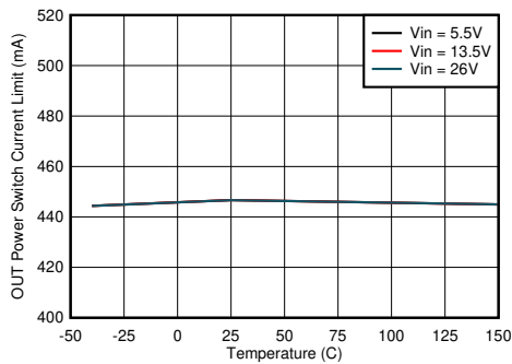
图 8-15. OUT Power Switch Current Limit vs Junction Temperature
