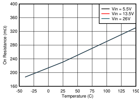
图 8-19. OUT Power Switch On Resistance vs Junction Temperature
