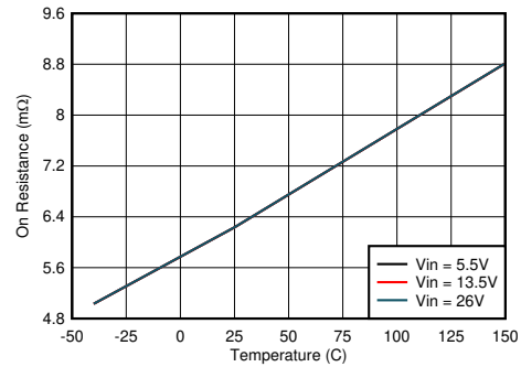
图 8-18. USB Power Switch On Resistance vs Junction Temperature
