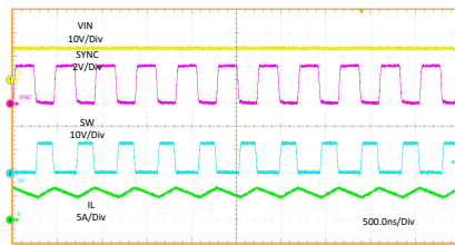
图 10-7. Switching Frequency When R_{FREQ} = 8.45 \text{ k}\Omega
