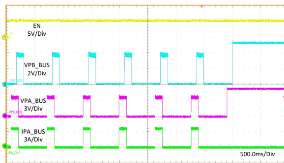
图 11-26. 1- \Omega Load Recovery
