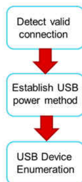
图 10-19. Flow of DFP-to-UFP Configuration
