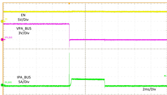
图 11-27. VBUS Hot Short to GND
