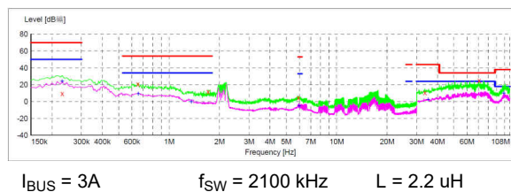
图 11-4. 2.1-MHz EMI Results (Without CM Filter)
