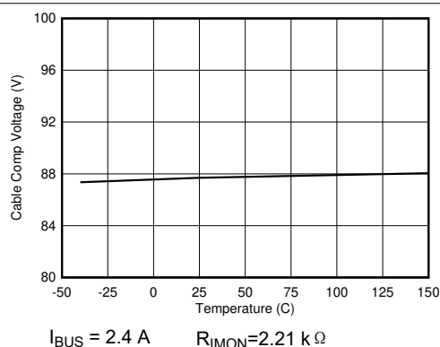
图 8-15. Cable Compensation Voltage vs Junction Temperature
