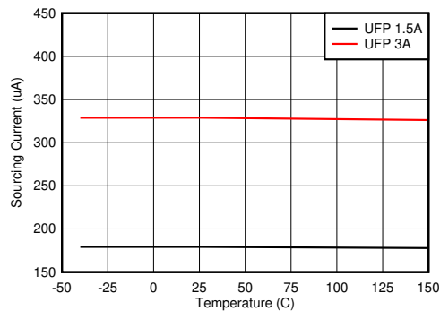
图 8-21. CC Sourcing Current vs Junction Temperature
