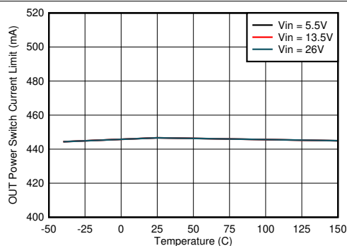
图 8-13. OUT Power Switch Current Limit vs Junction Temperature
