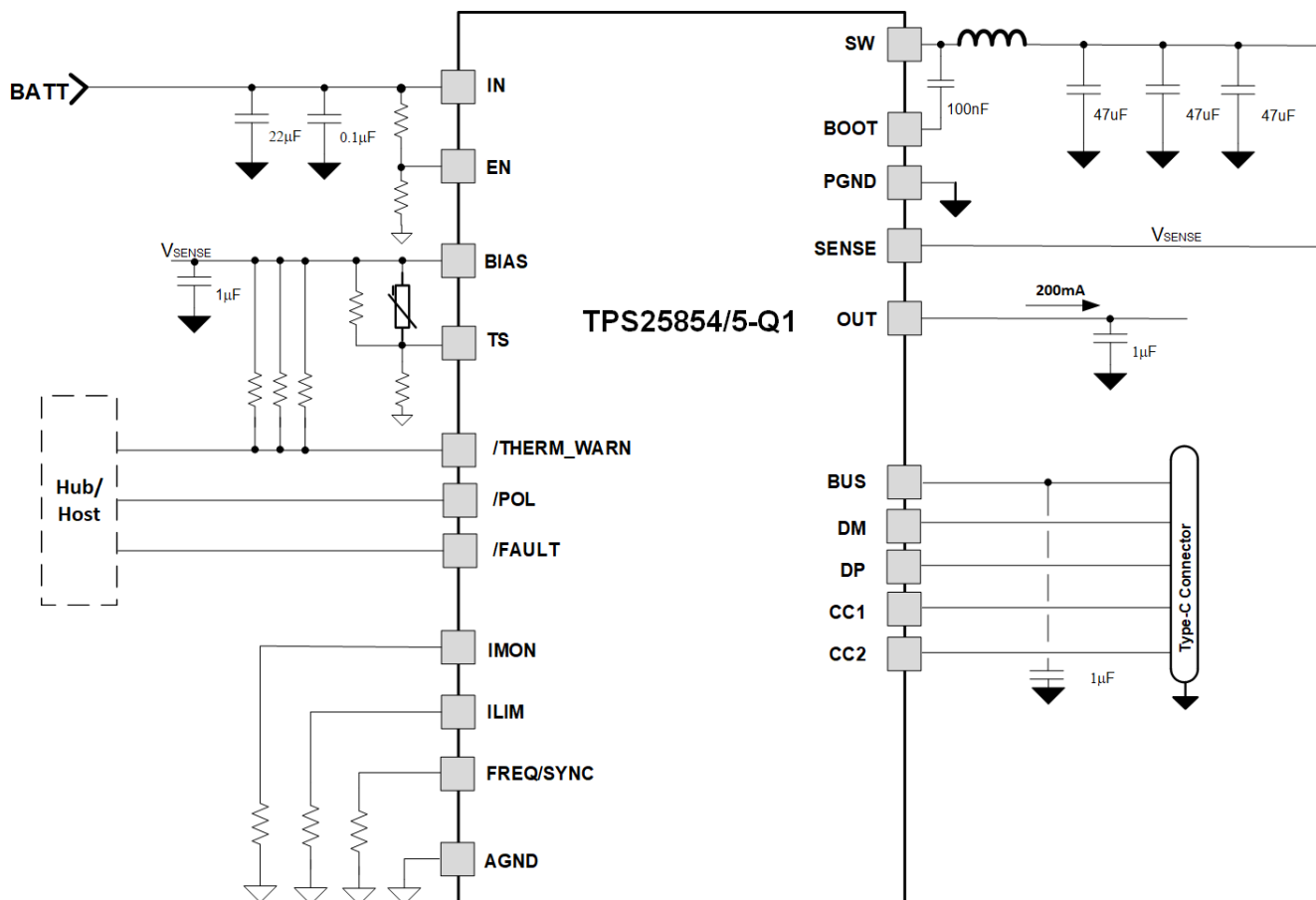
图 11-1. TPS2585x-Q1 Typical Application Circuit for 400-KHz f_{sw}
