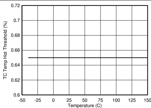
图 8-23. TS Temperature Hot Threshold vs Junction Temperature
