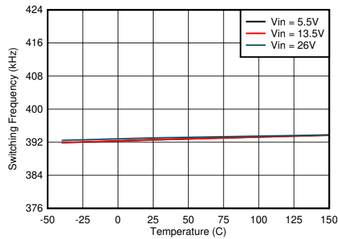
图 8-19. Switching Frequency vs Junction Temperature
