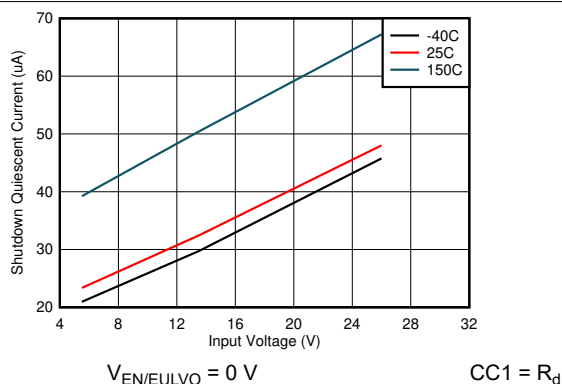
图 8-1. Shutdown Quiescent Current
