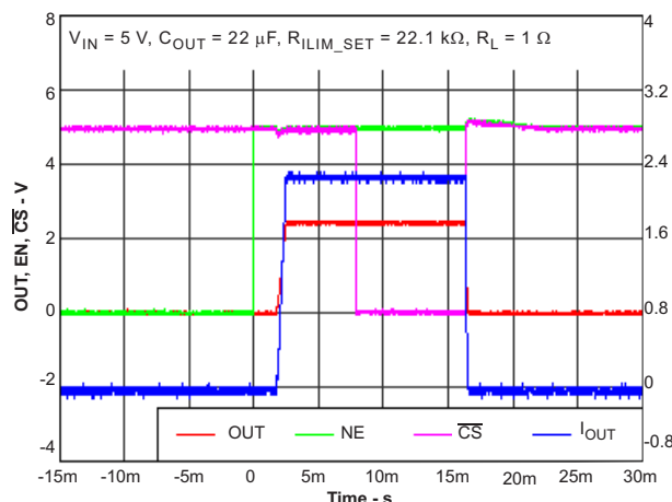
Figure 14. Enable into 1- \Omega Load
