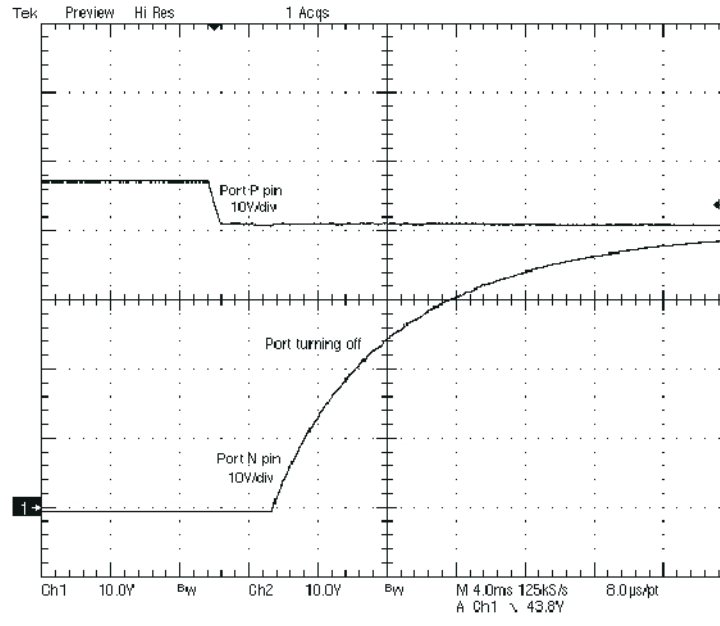
图 8-8. Port Turn OFF due to Undervoltage Fault
