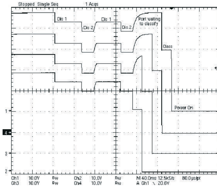
图 8-5. Four Port Discovery, Class, Power On
