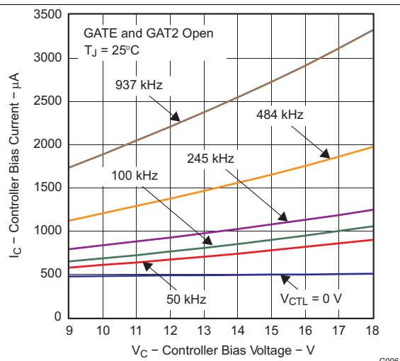
Figure 9. '754 Controller Bias Current vs Voltage
