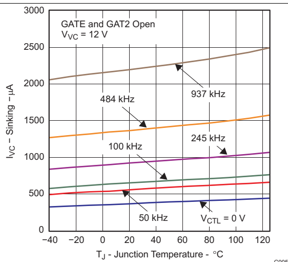
Figure 8. Controller Bias Current vs Temperature
