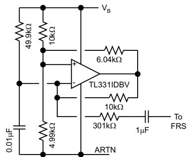
Figure 36. Frequency Dithering
