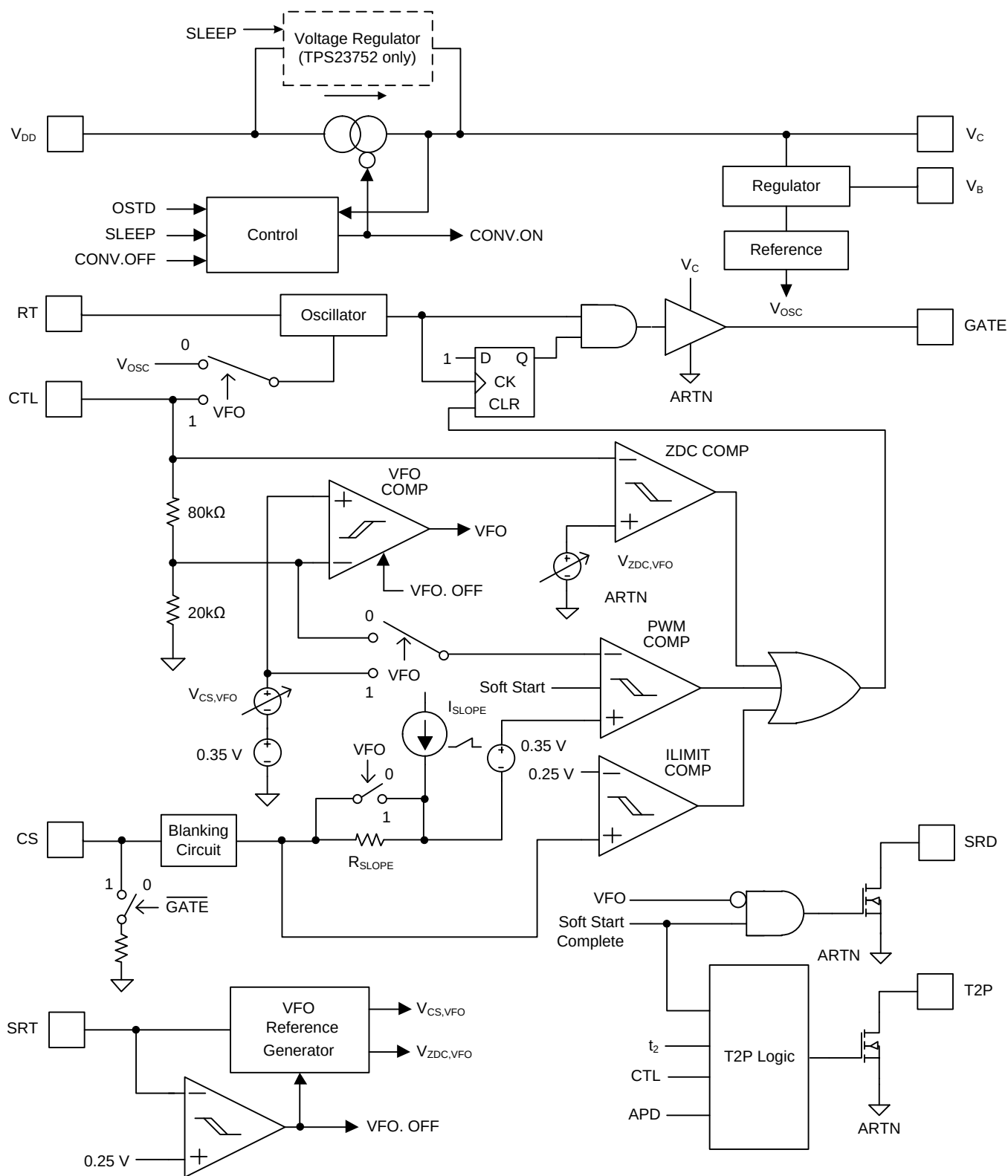
Figure 20. DC-DC Controller
