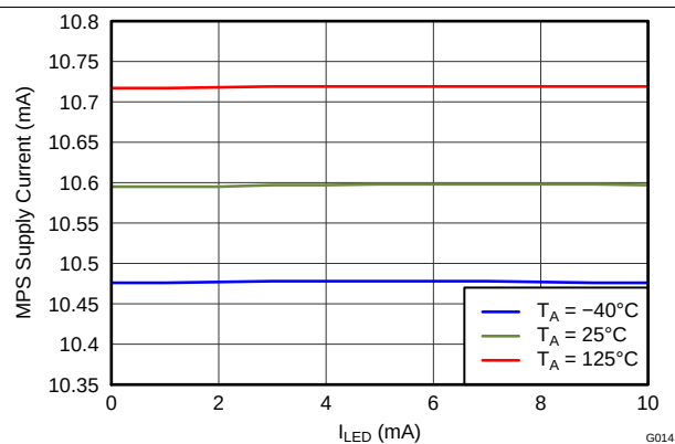
Figure 18. MPS Supply Current vs LED Current
