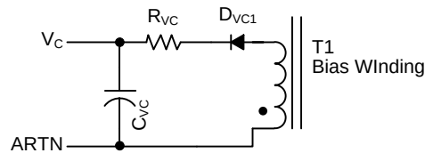
Figure 34. V_{\text{C}} Pin Interface
