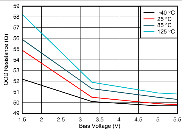
图 6-2. QOD-Resistance vs Bias Voltage
