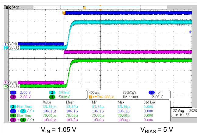
图 6-45. Turnon Response Time
