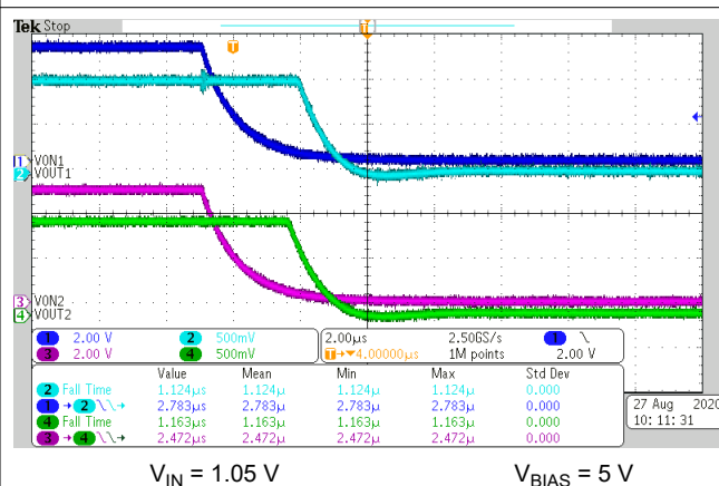
图 6-46. Turnoff Response Time
