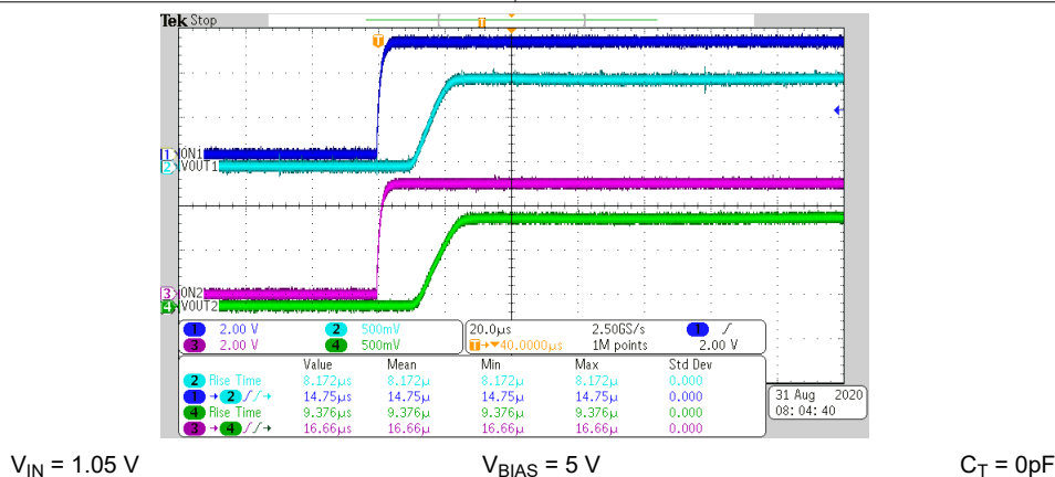
图 6-47. Turnon Response Time
