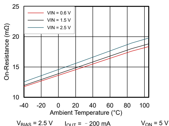
图 6-10. On-Resistance vs Ambient Temperature Single Channel (TPS22976)
