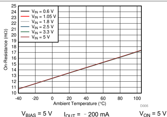
图 6-12. On-Resistance vs Ambient Temperature Single Channel (TPS22976A, TPS22976N)
