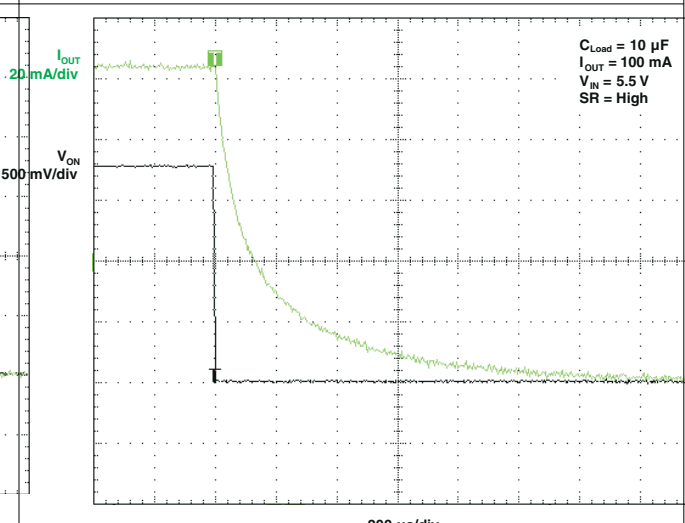
图 5-19. t_{OFF} Response
