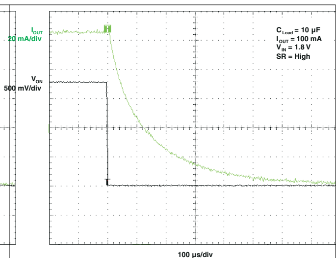
图 5-17. t_{OFF} Response
