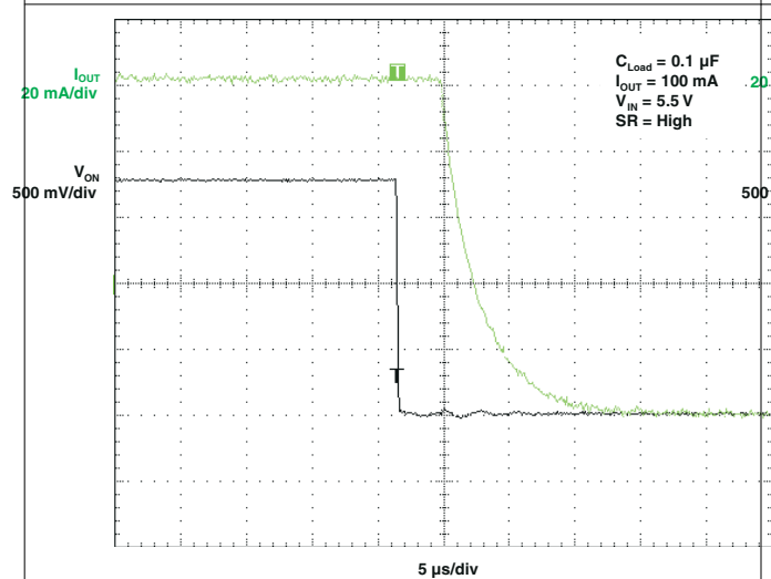
图 5-18. t_{OFF} Response
