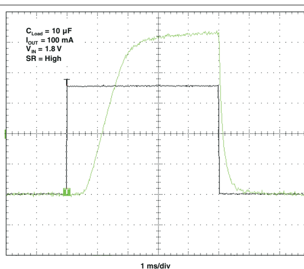
图 5-13. t_{ON} Response
