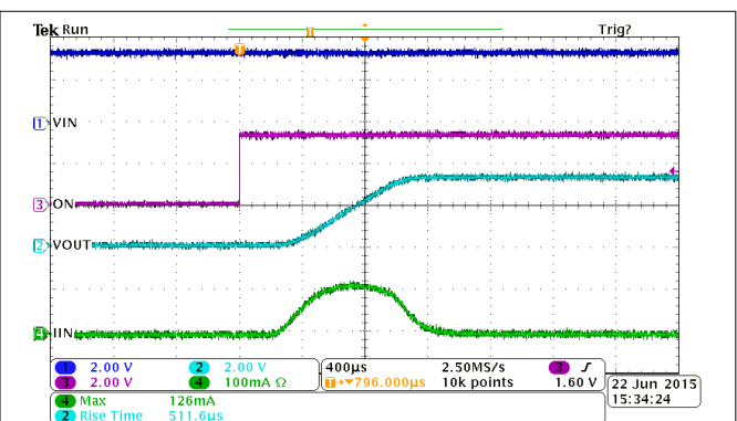
图 8-3. Inrush Current with SR = High
