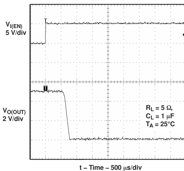
图 6-31. Turnoff Delay and Fall Time With 1-μF Load
