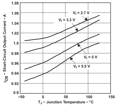
图 6-10. Short-Circuit Output Current vs Junction Temperature
