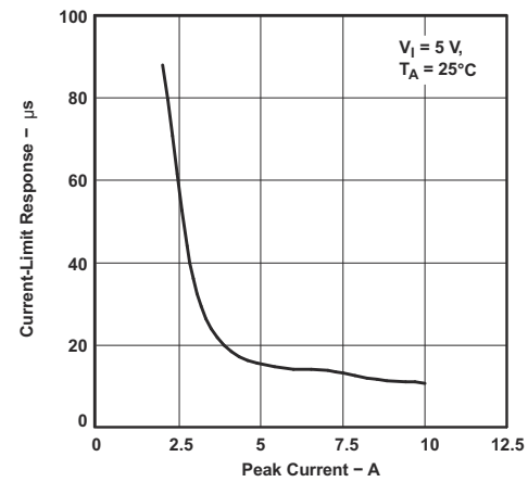
图 6-12. Current-Limit Response vs Peak Current
