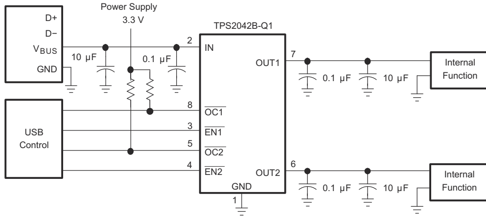
图 9-14. High-Power Bus-Powered Function (TPS2042B-Q1)
