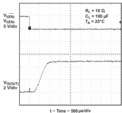
图 9-5. Turnon Delay and Rise Time With 100-μF Load
