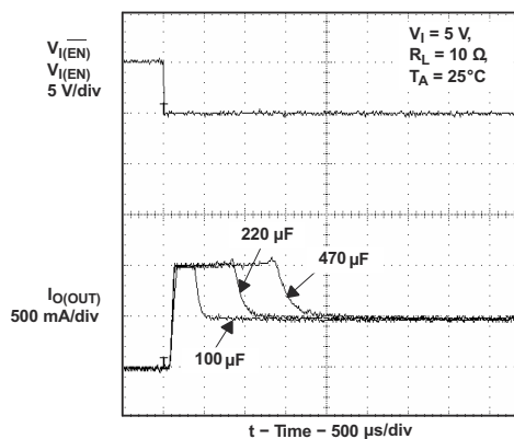
图 9-8. Inrush Current With Different Load Capacitance
