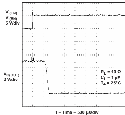
图 9-4. Turnoff Delay and Fall Time With 1-μF Load
