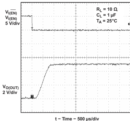
图 9-3. Turnon Delay and Rise Time With 1-μF Load
