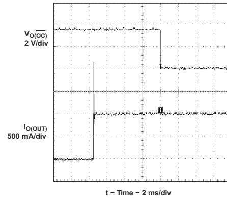
图 9-10. 2-Ω Load Connected to Enabled Device
