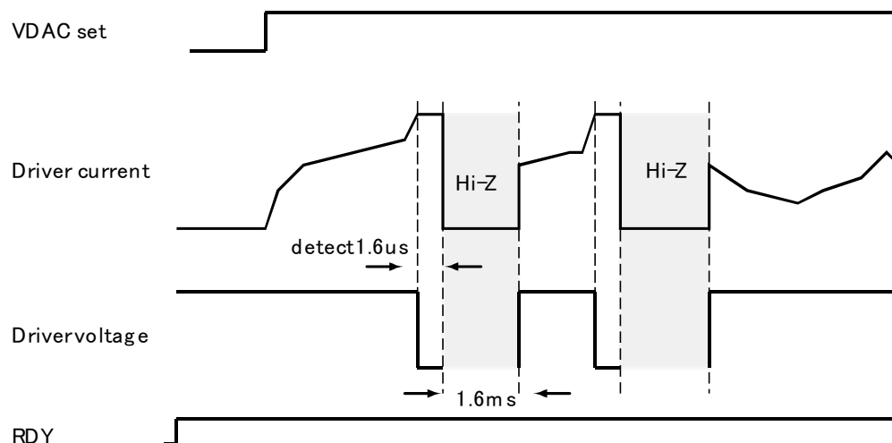
Figure 7. Example of SCP (Driver Short to GND)
