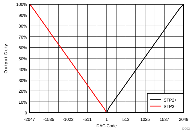
Figure 5. STP2 Driver: DAC Code vs Output On Duty
