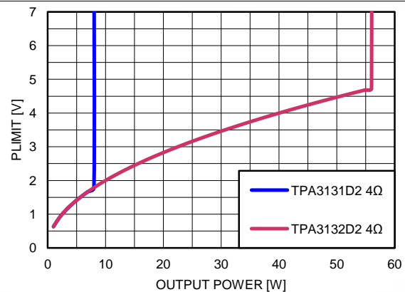
Figure 23. PLIMIT vs. Max. Output Power, 4Ω load
