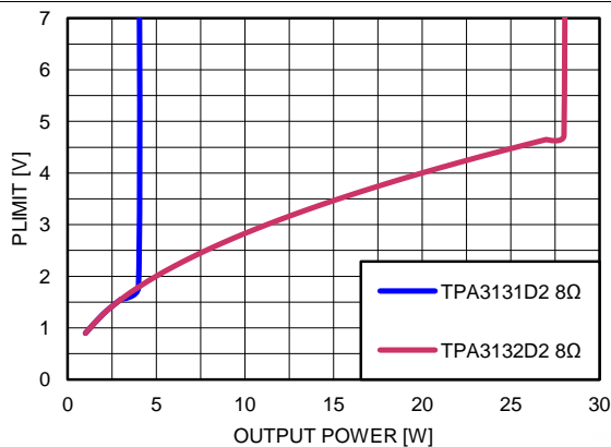
Figure 22. PLIMIT vs. Max. Output Power, 8Ω load
