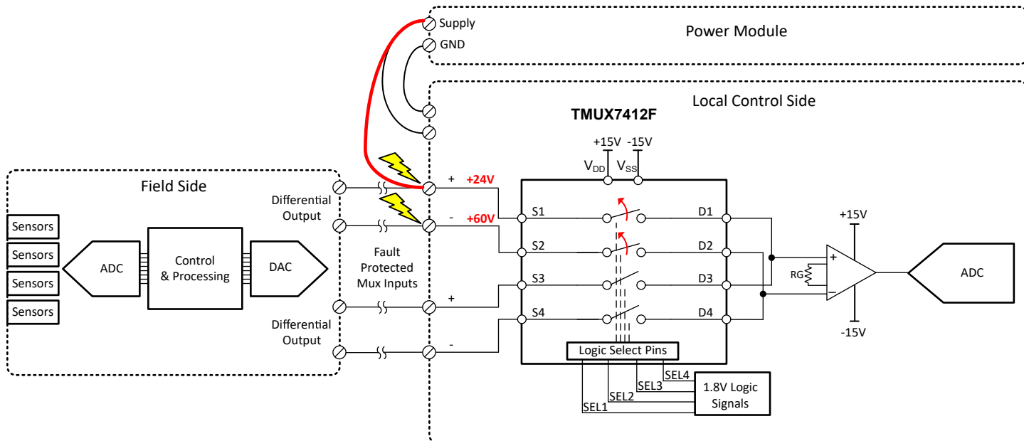
图 10-1. Typical Application
