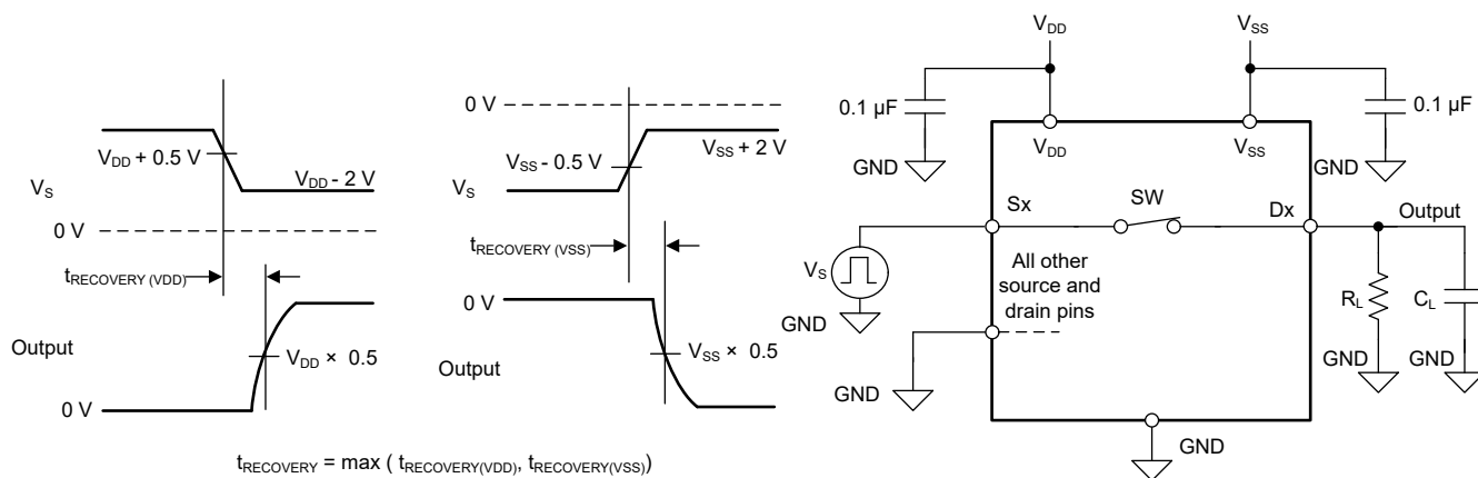
图 8-8. Fault Recovery Time Measurement Setup
