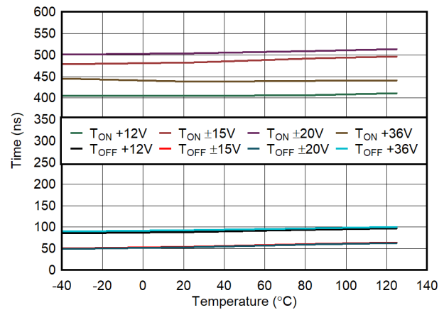
图 7-28. t_{ON} and t_{OFF} vs Temperature
