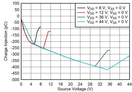
图 7-26. Charge Injection vs Source Voltage - Single Supply
