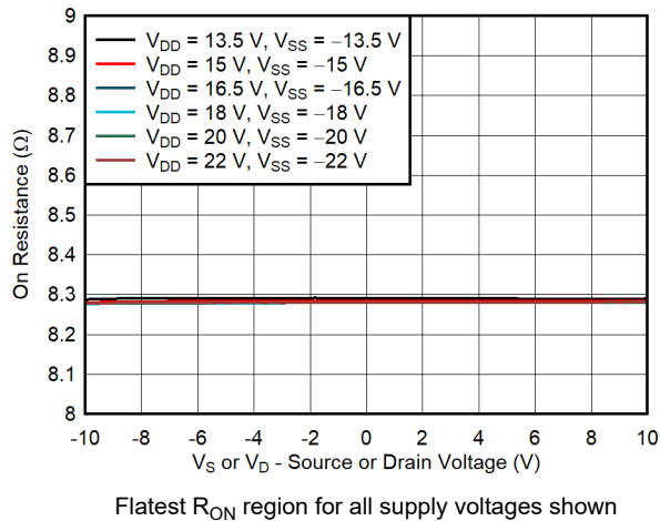
图 7-3. On-Resistance vs Source or Drain Voltage
