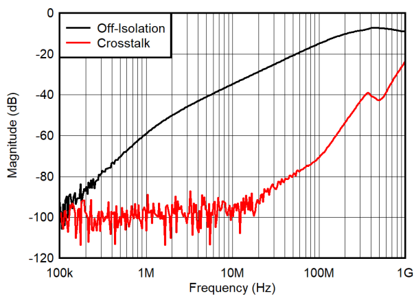
图 7-29. Crosstalk and Off Isolation vs Frequency
