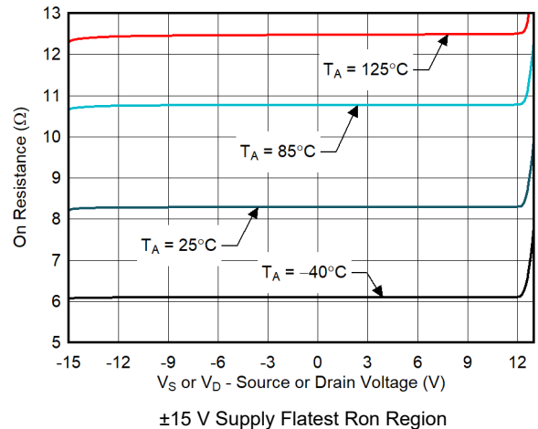
图 7-4. On-Resistance vs Source or Drain Voltage
