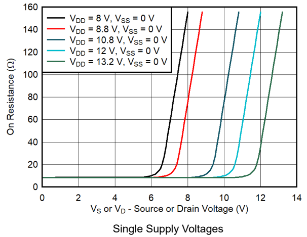
图 7-6. On-Resistance vs Source or Drain Voltage
