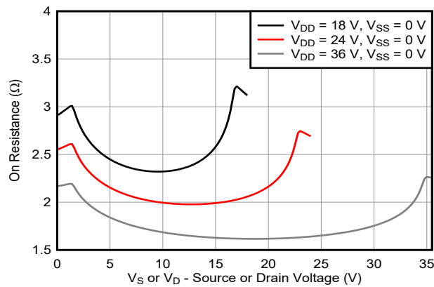
图 5-1. On-Resistance vs Source or Drain Voltage - Dual Supply
