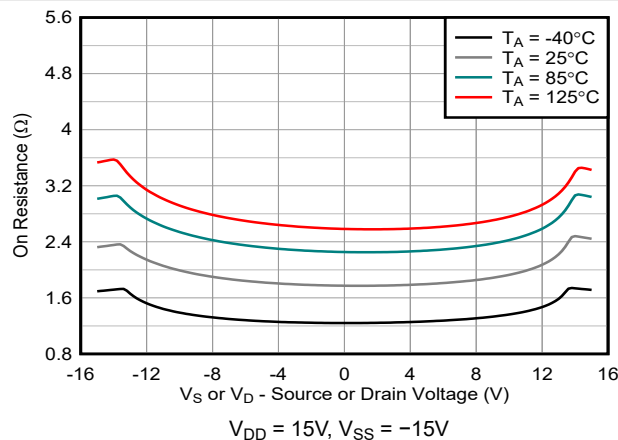
图 5-5. On-Resistance vs Temperature
