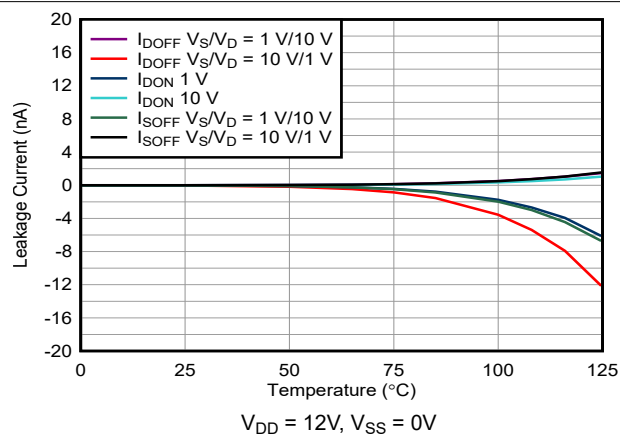
图 5-10. On-Leakage vs Temperature
