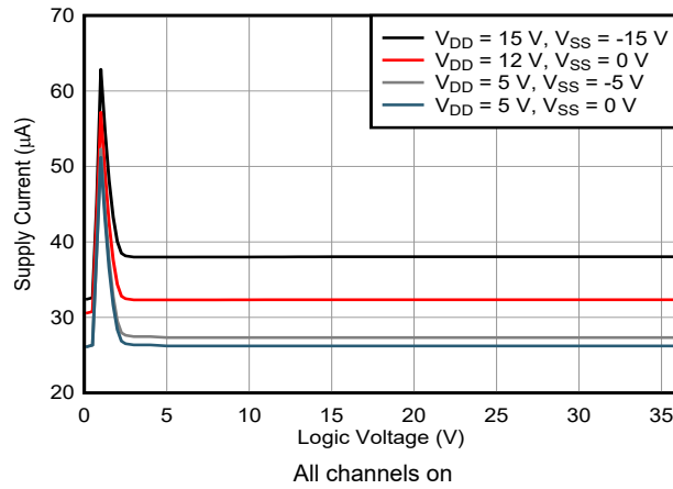
图 5-13. Supply Current vs Logic Voltage
