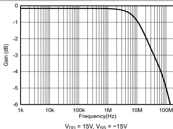
图 5-24. On Response vs Frequency
