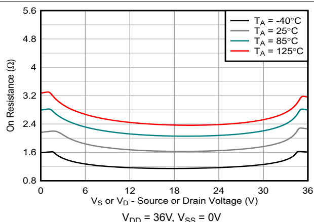
图 5-8. On-Resistance vs Temperature
