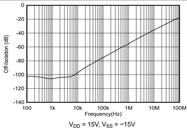
图 5-22. Off-Isolation vs Frequency
