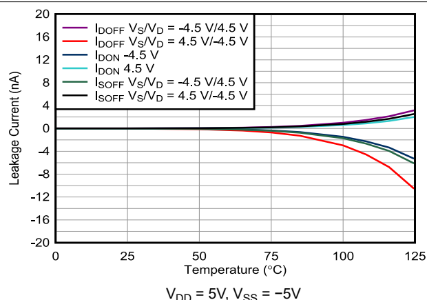
图 5-12. On-Leakage vs Temperature
