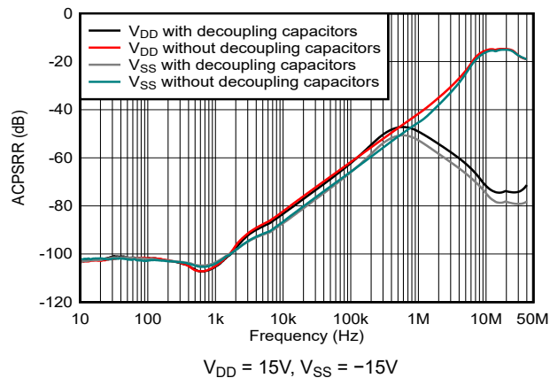
图 5-29. ACPSRR vs Frequency
