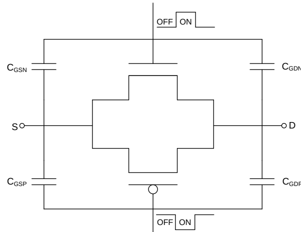
图 30. Transmission Gate Topology
