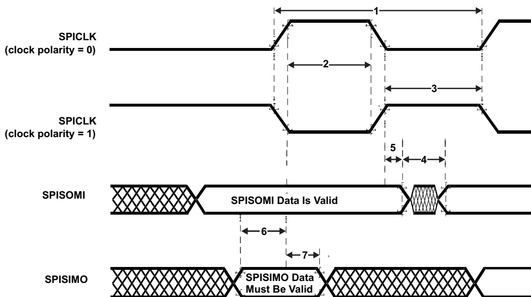
图 7-12. SPI Slave Mode External Timing (CLOCK PHASE = 1)
