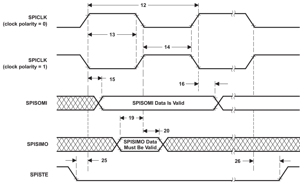
图 4-71. SPI Slave Mode External Timing (Clock Phase = 0)
