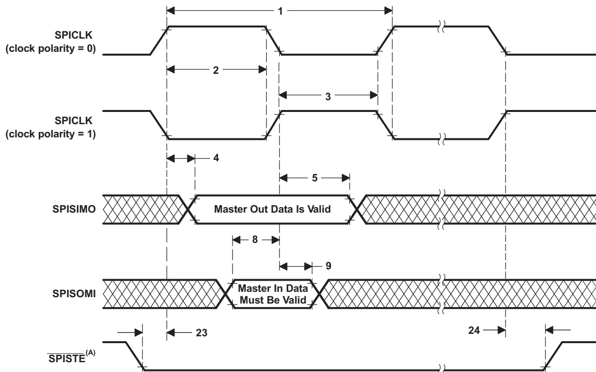
图 4-73. High-Speed SPI Master Mode External Timing (Clock Phase = 0)
