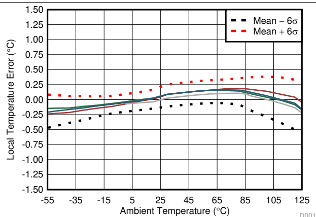
图 2. Local Temperature Error vs Ambient Temperature
