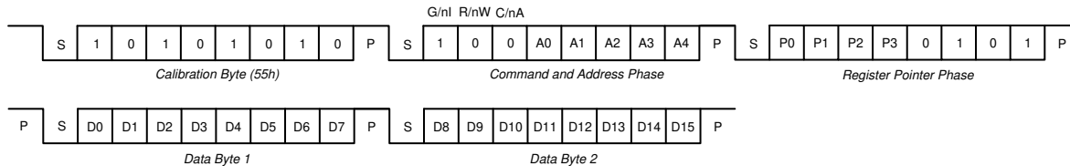
Figure 28. Global Write Operation
