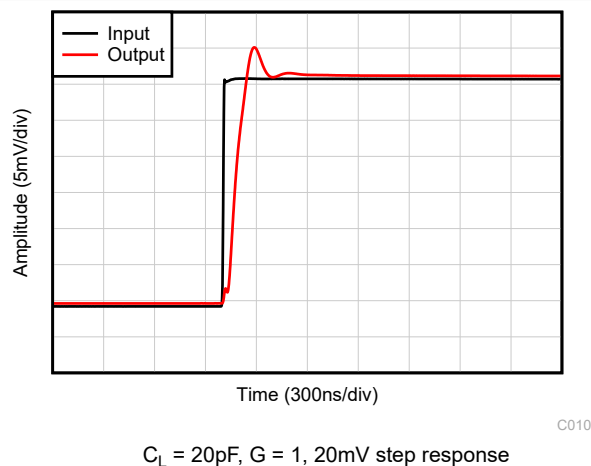
Figure 5-33. Small-Signal Step Response, Rising
