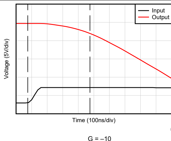
Figure 5-31. Positive Overload Recovery
