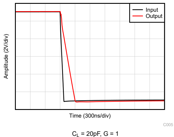
Figure 5-36. Large-Signal Step Response (Falling)
