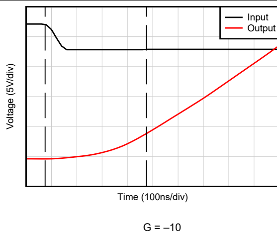
Figure 5-32. Negative Overload Recovery
