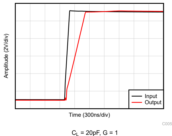
Figure 5-35. Large-Signal Step Response (Rising)
