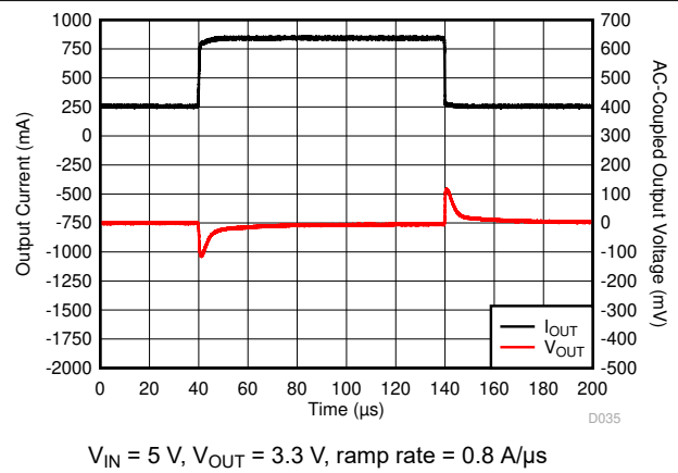
图 6-12. I_{OUT} Transient From 250 mA to 850 mA
