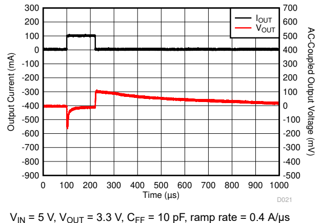
图 6-10. I_{OUT} Transient From 0 mA to 100 mA
