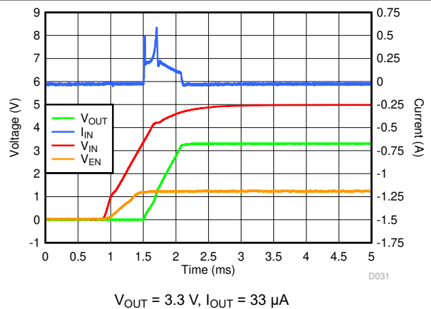
图 6-34. Startup Inrush Current With C_{OUT} = 47\text{ }\mu\text{F}
