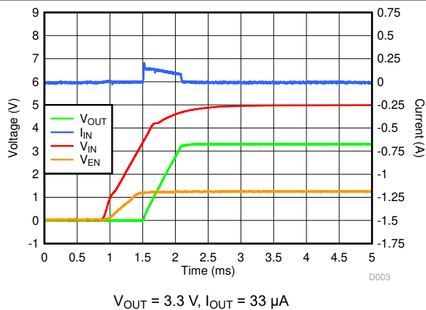
图 6-33. Startup Inrush Current With C_{OUT} = 22\text{ }\mu\text{F}
