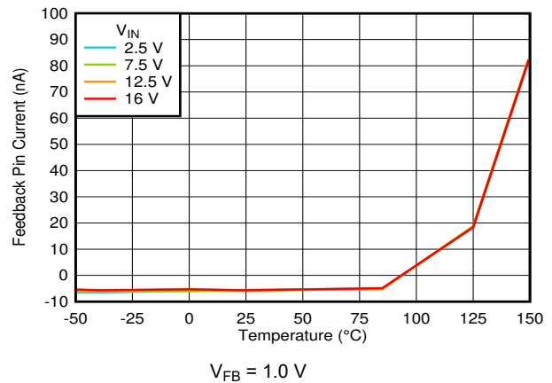
图 6-32. I_{FB} vs Temperature
