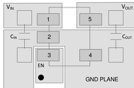
● Represents via used for application specific connections 图 11-5. Layout Example for the Fixed DBV Version
