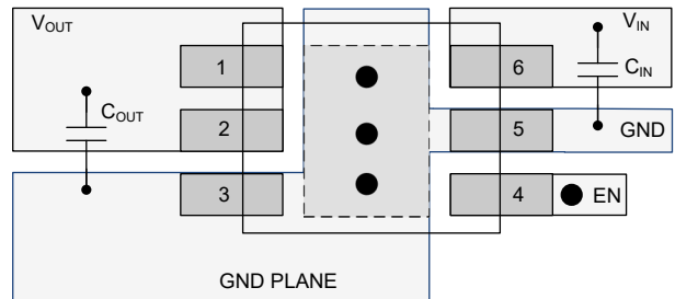
● Represents via used for application-specific connections 图 11-2. Layout Example for the Fixed WSON Version
