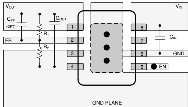
● Represents via used for application-specific connections 图 11-2. Layout Example for the Fixed WSON Version
