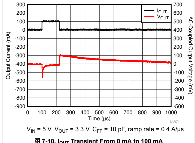
图 7-10. I_{OUT} Transient From 0\text{ mA} to 100\text{ mA}
